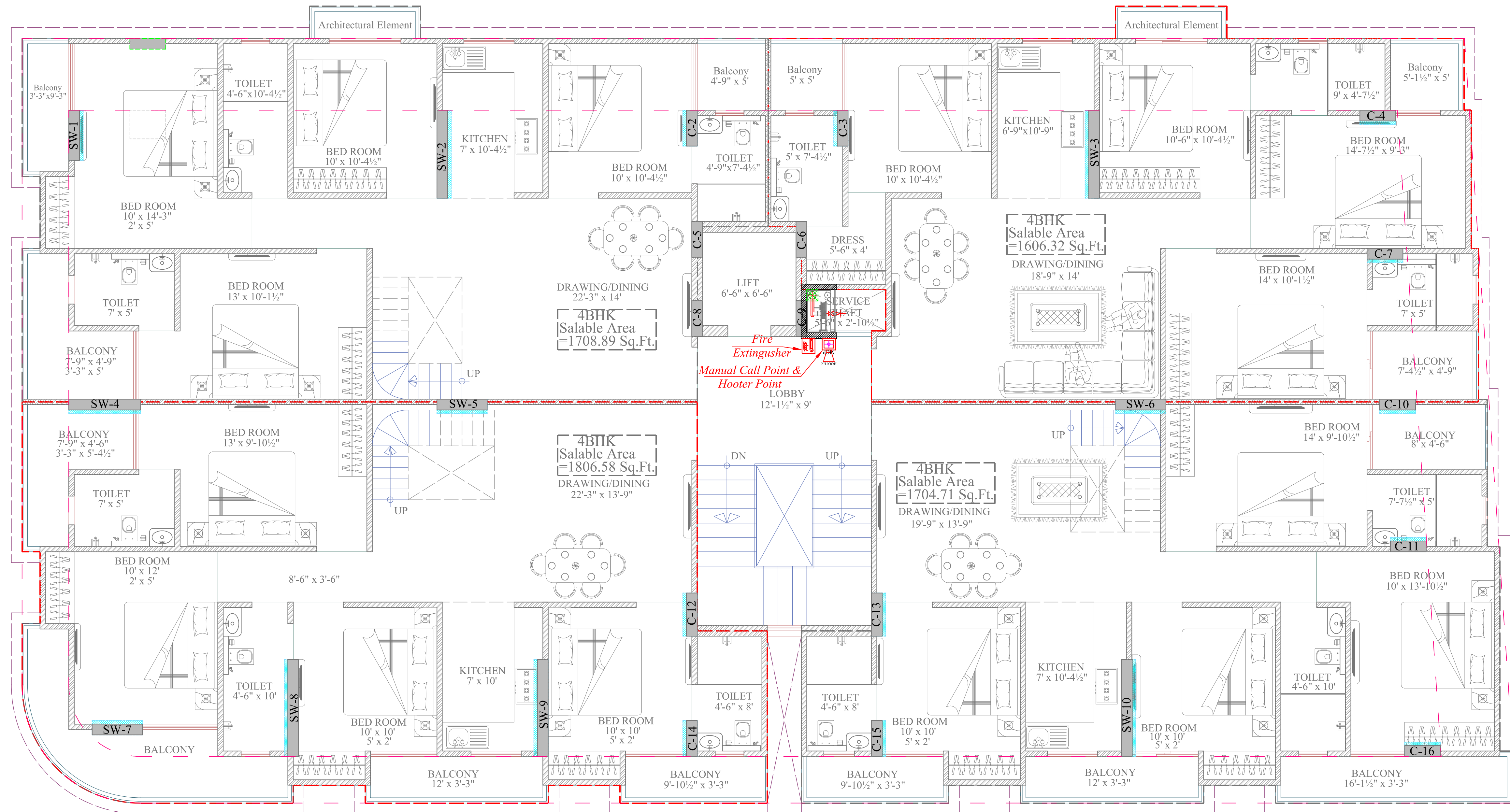
6th FLOOR PLAN
