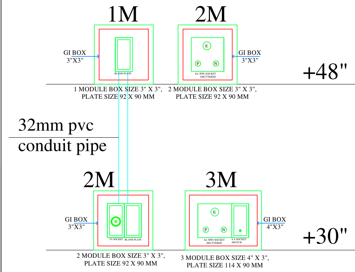
TYPICAL TV WALL ELEVATION PLAN
