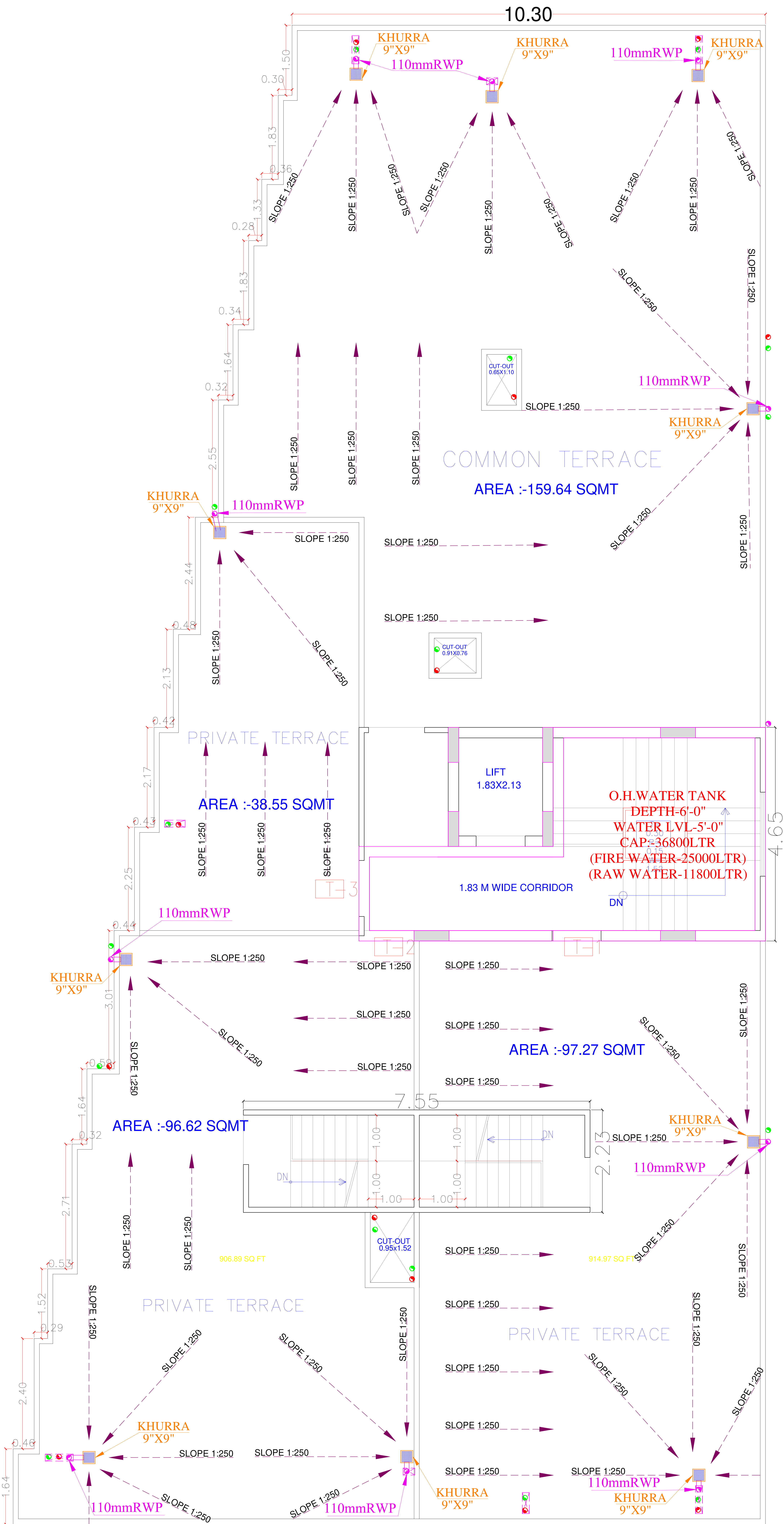
TERRACE FLOOR PLAN
