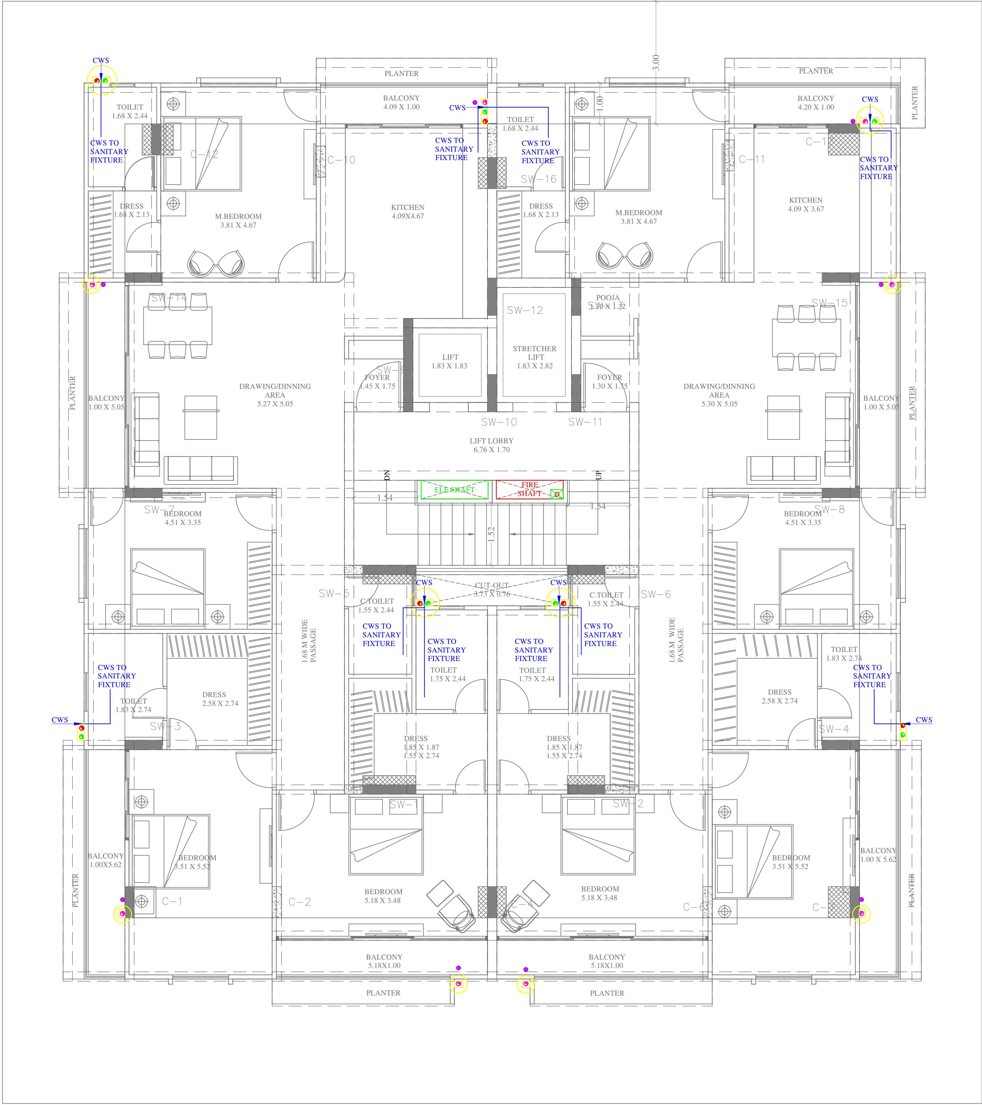
TYPICAL FLOOR [FIRST TO FIFTH]
