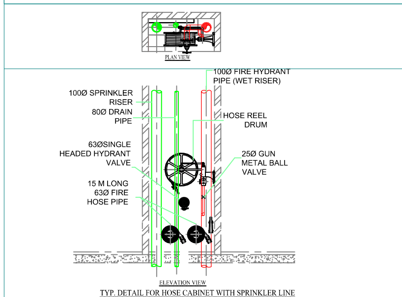
DRAWING: TYP. DETAIL FOR FIRE CABINET FHC-2
