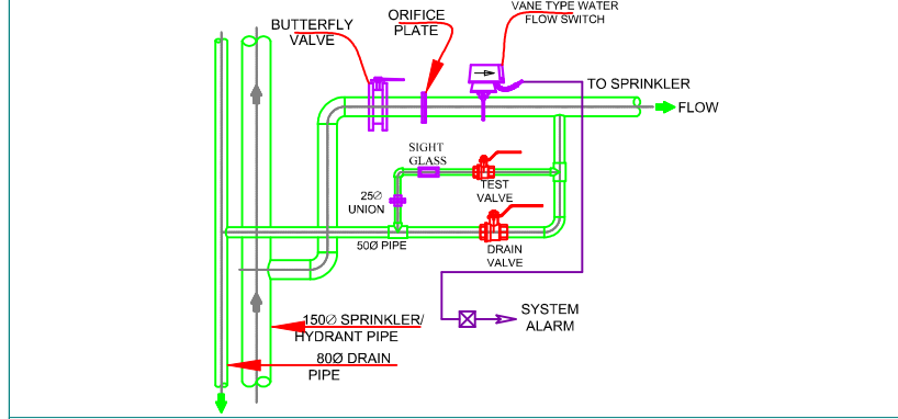
DRAWING: TYP. DETAIL FOR FIRE FIGHTING HORIZONTAL PIPEING & CLAMP
