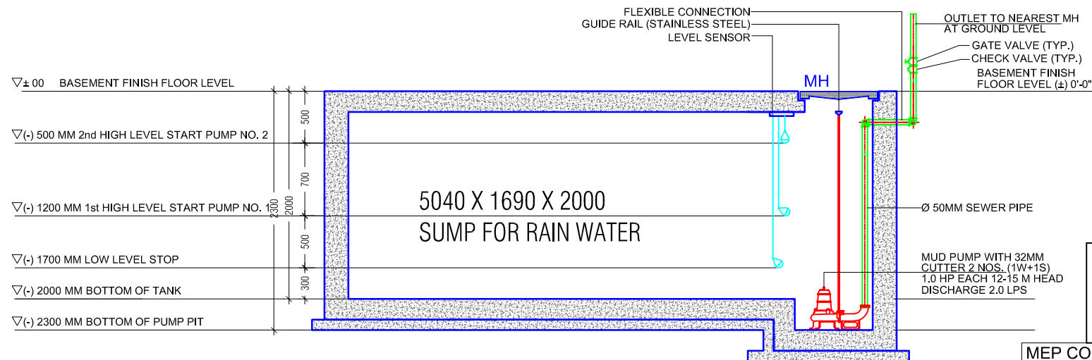
SUMP SECTION AA
