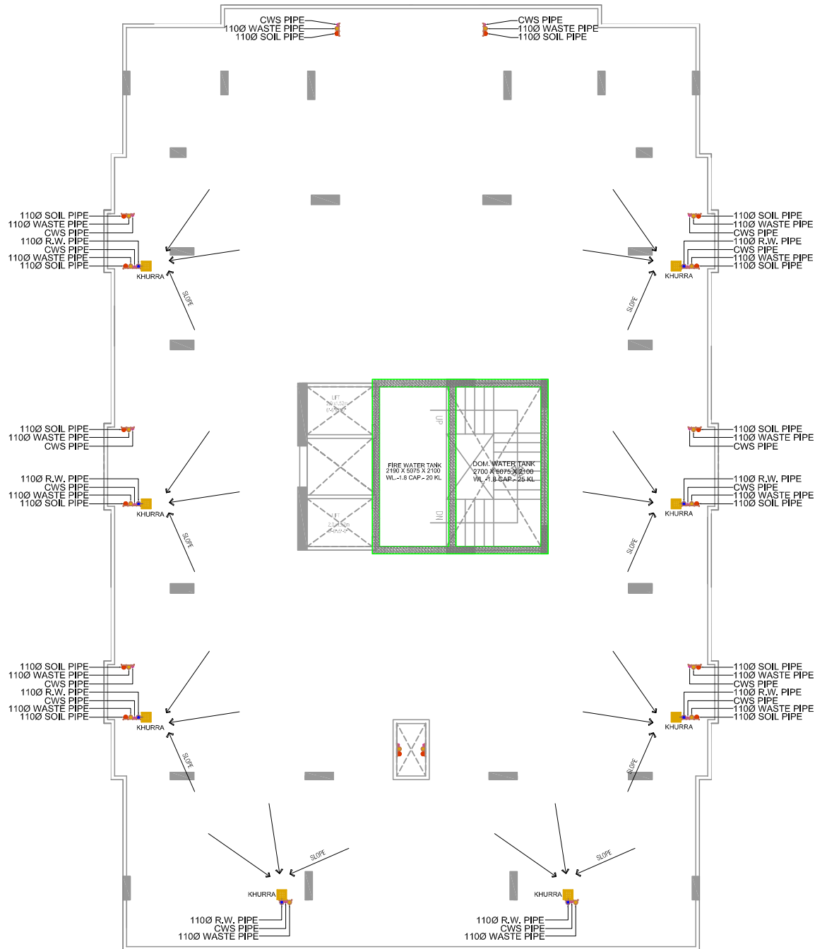
TERRACE FLOOR DRAINAGE LAYOUT
