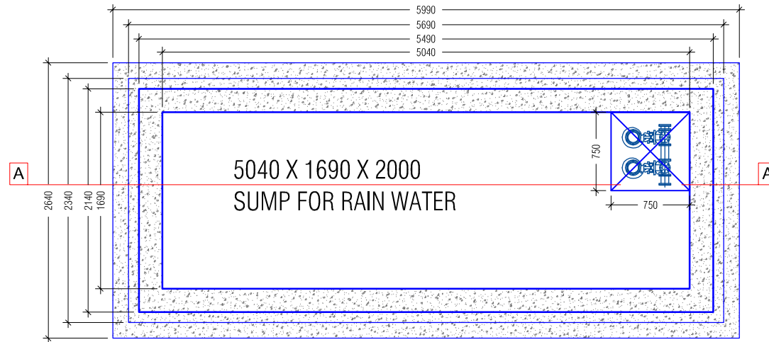
SUMP PLAN
