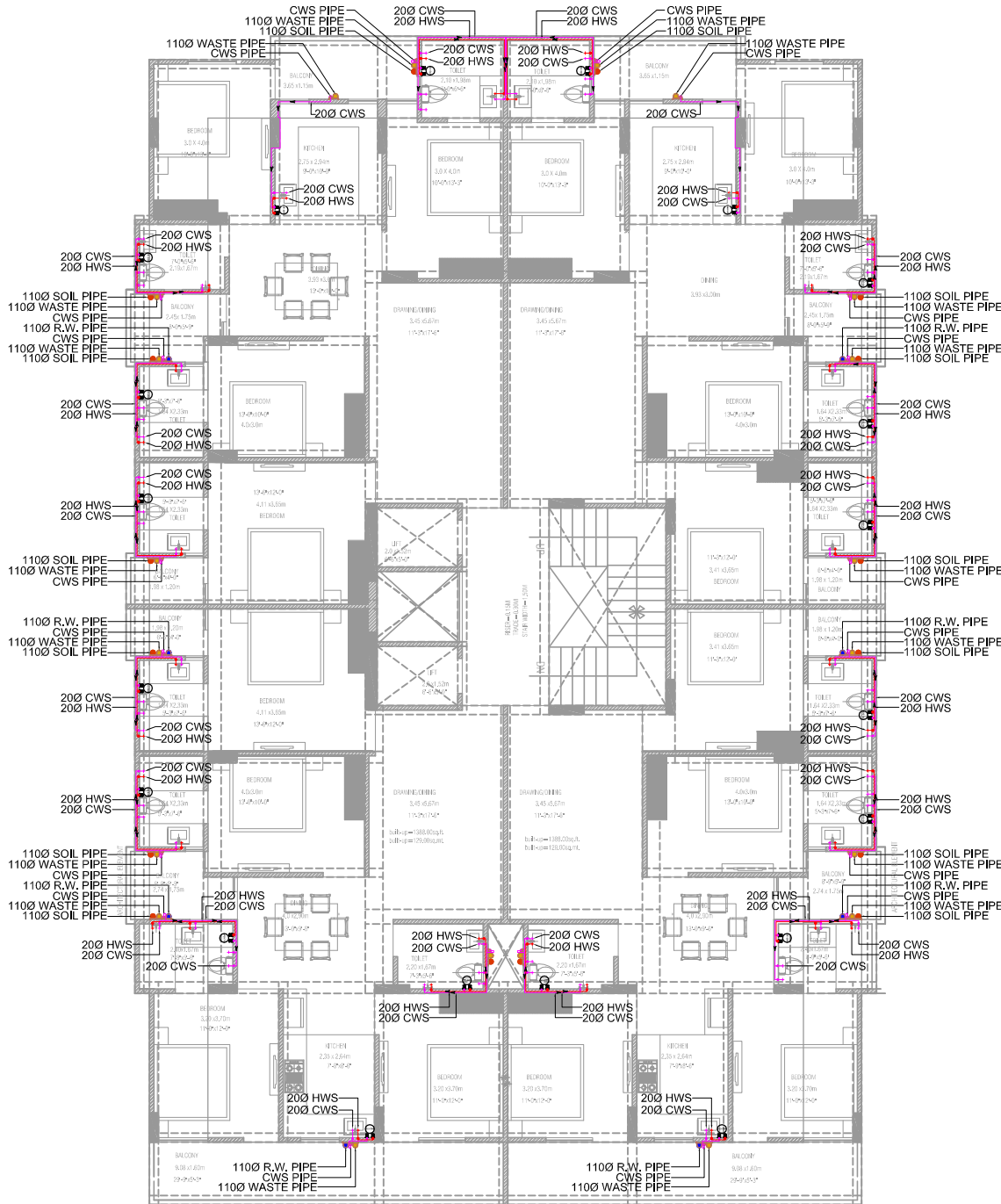
TYPICAL FLOOR PLUMBING LAYOUT
