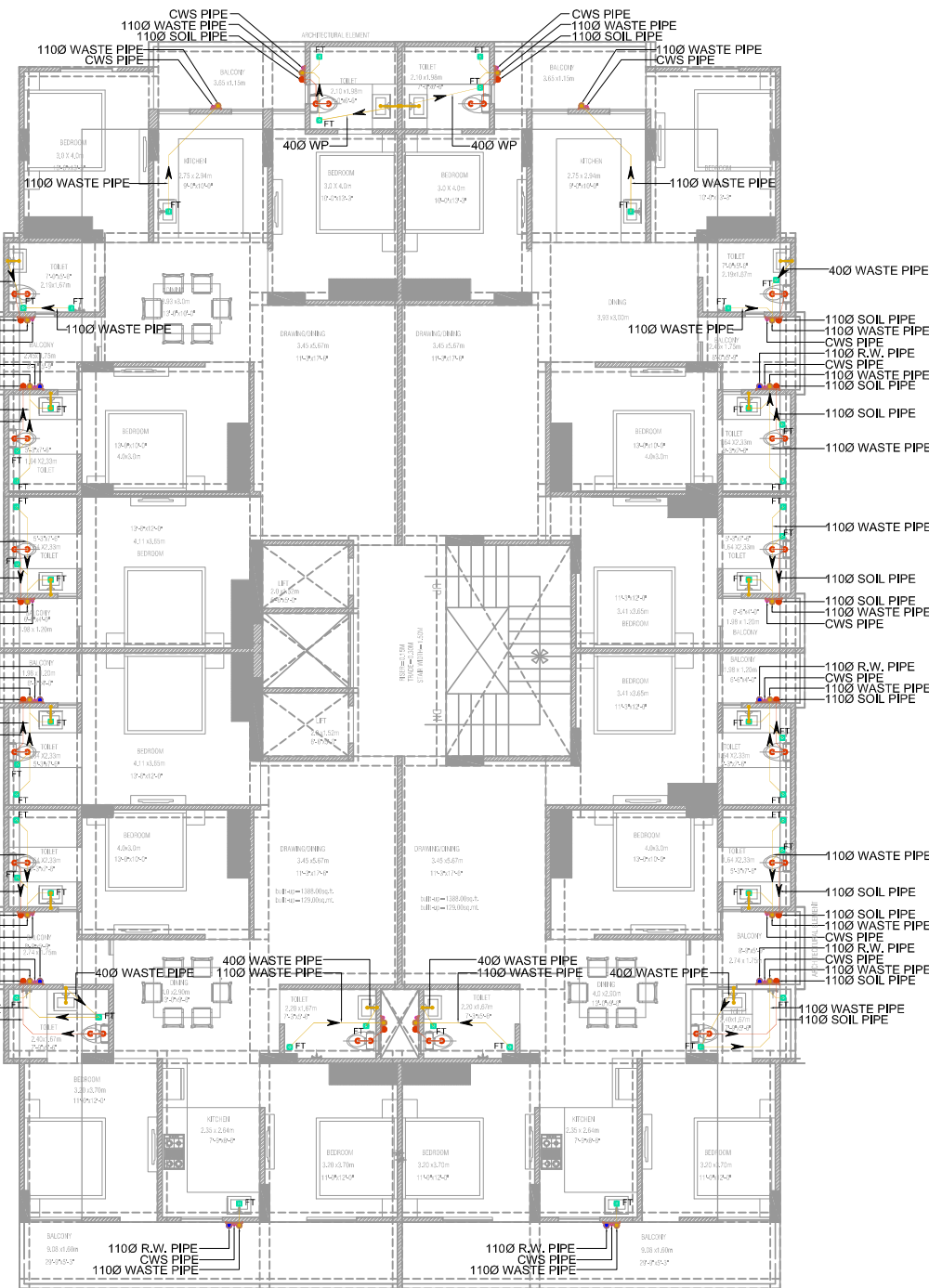
TYPICAL FLOOR DRAINAGE LAYOUT
