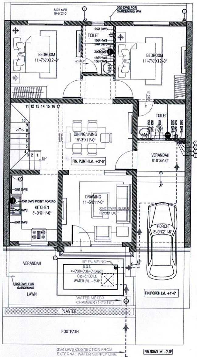
GROUND FLOOR WATER SUPPLY LAYOUT PLAN
