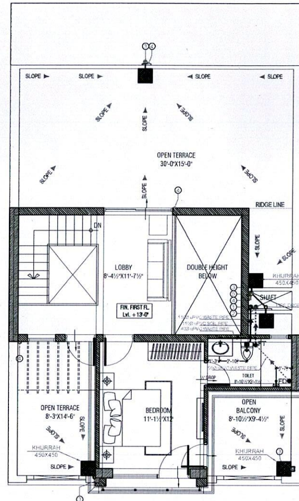
FIRST FLOOR DRAINAGE LAYOUT PLAN
