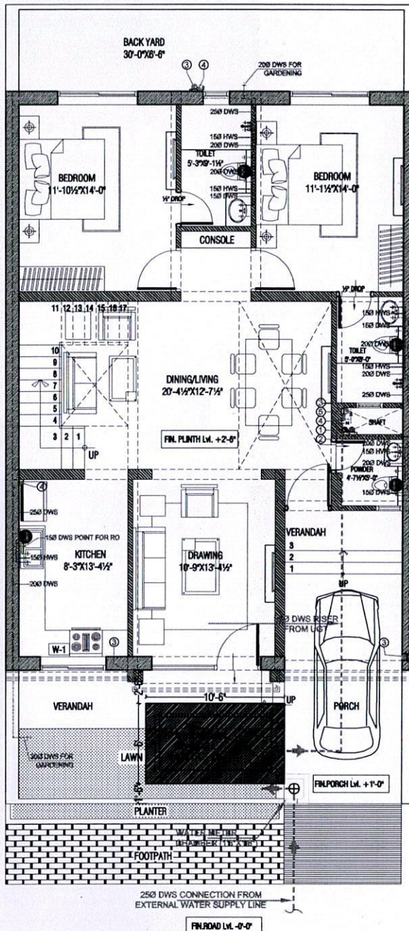
GROUND FLOOR WATER SUPPLY LAYOUT PLAN
