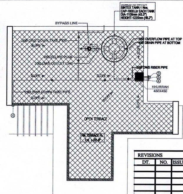
TERRACE PLUMBING LAYOUT PLAN
