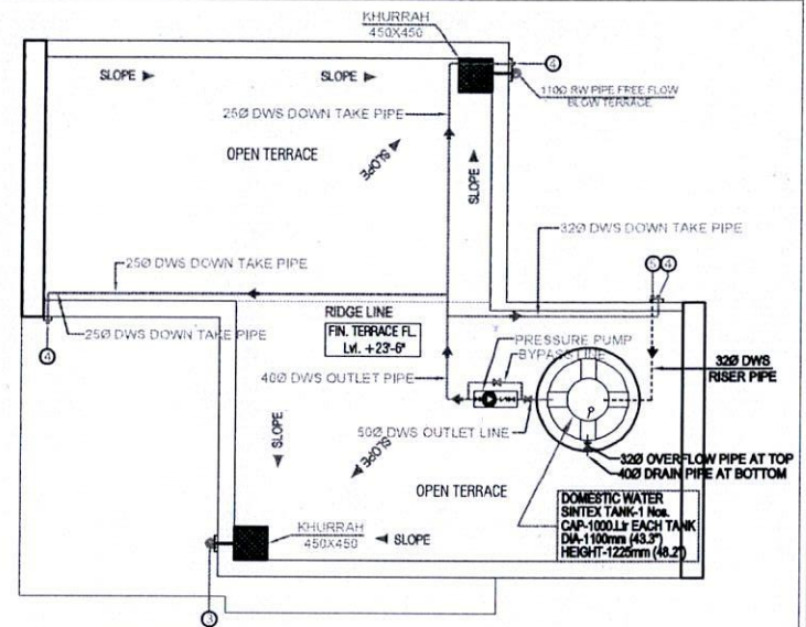
TERRACE PLUMBING LAYOUT PLAN
