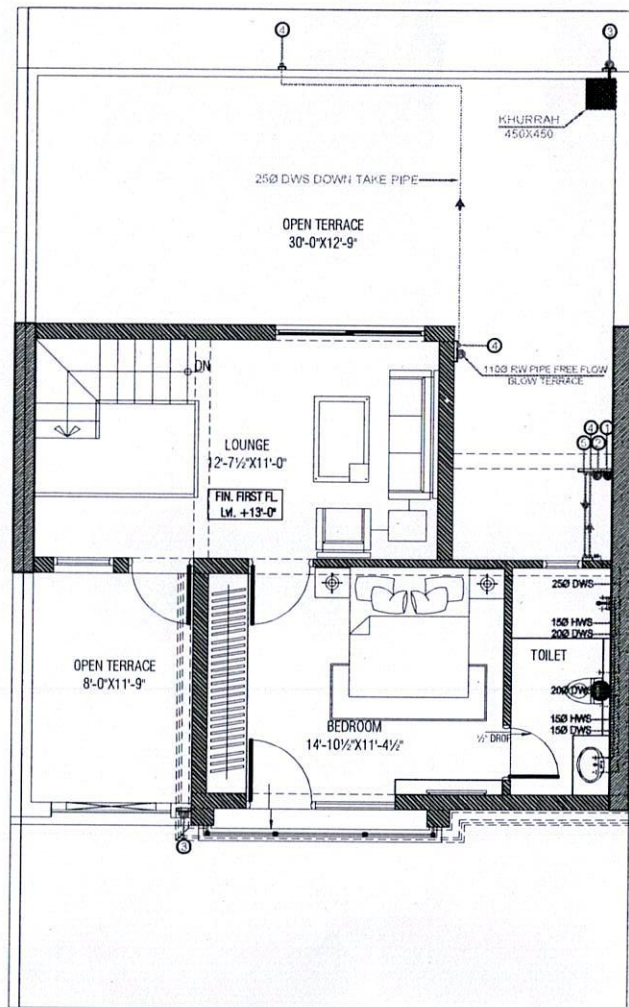
FIRST FLOOR WATER SUPPLY LAYOUT PLAN
