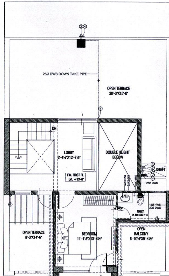
FIRST FLOOR WATER SUPPLY LAYOUT PLAN
