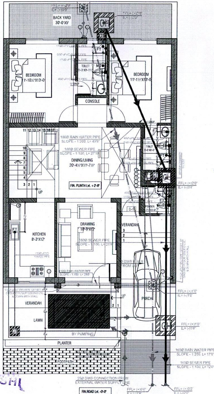
GROUND FLOOR DRAINAGE LAYOUT PLAN
