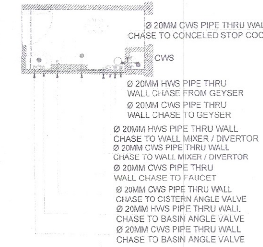
TYPICAL TOILET INTERNAL PLUMBING PLAN
