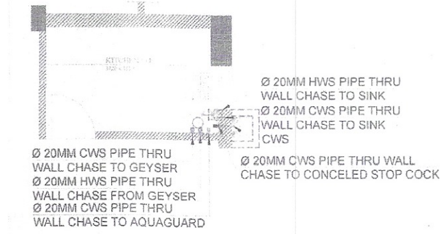
TYPICAL KITCHEN INTERNAL PLUMBING PLAN
