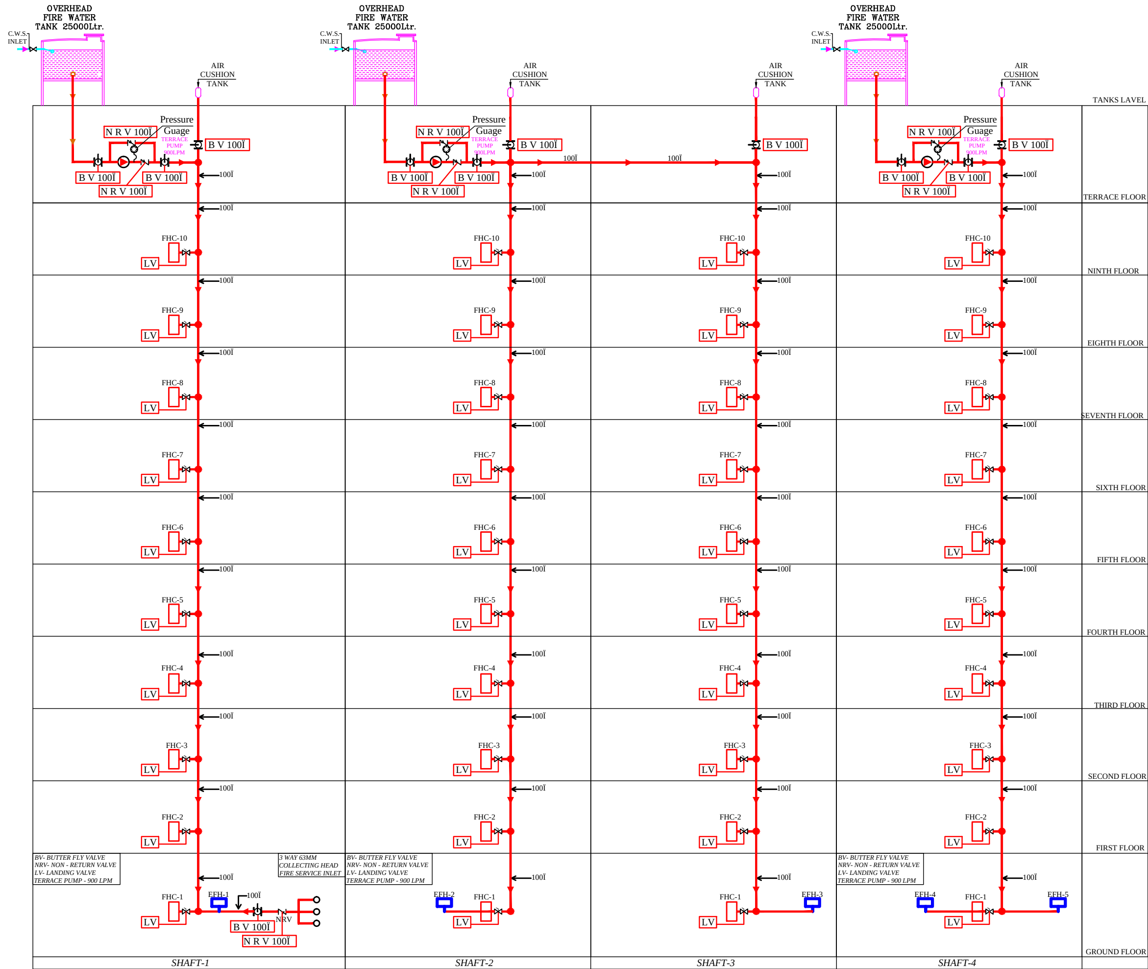
DRAWING TITLE:- FIRE SCHEMATIC LAYOUT
