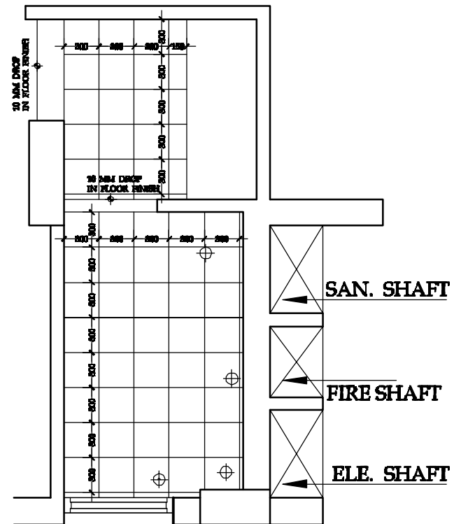
FLOORING DETAIL
