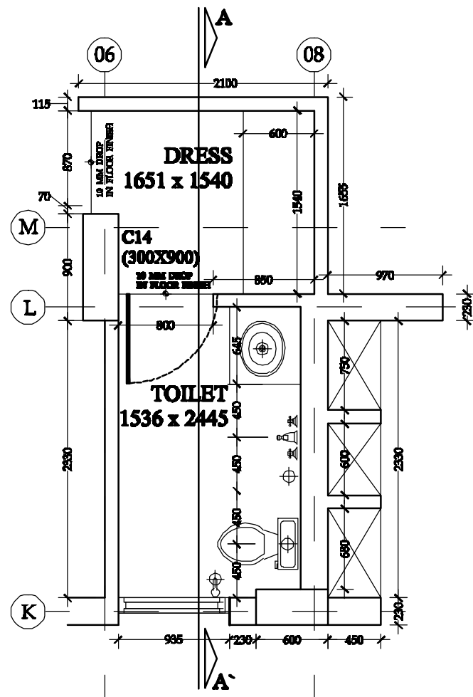
PLAN
