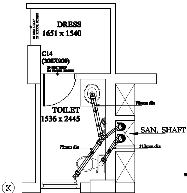
PIPE DETAIL
