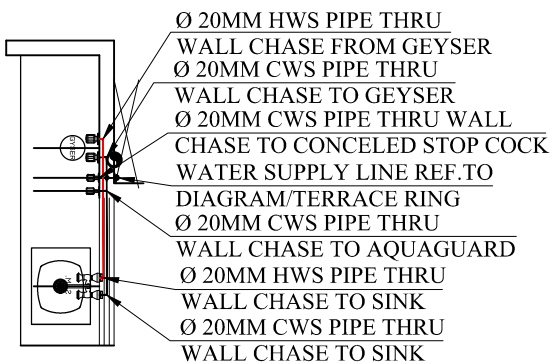
TYPICAL KITCHEN INTERNAL PLUMBING DETAIL
