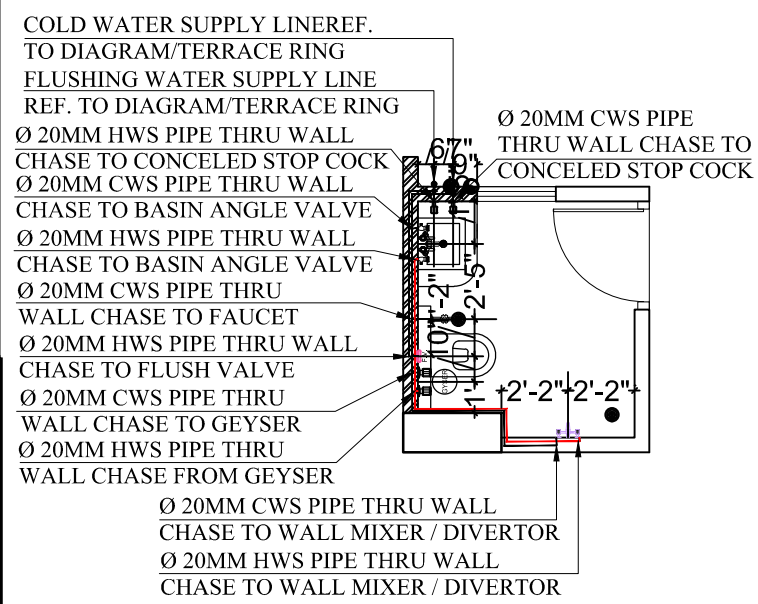
TYPICAL TOILET INTERNAL PLUMBING DETAIL
