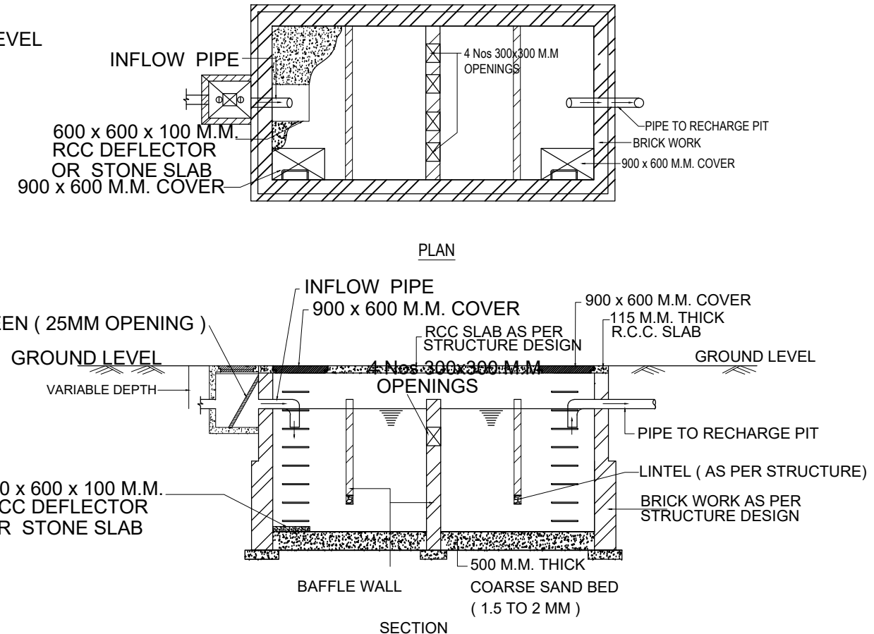
DESILTING / SETTLING CHAMBER
