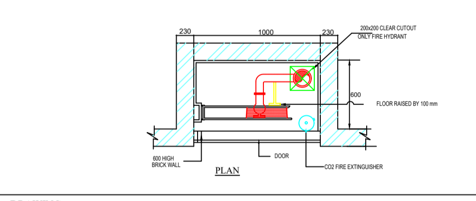
DRAWING: TYPICAL DETAIL FOR FIRE HYDRANT CABINET SCALE: 1:5 FIG-1
