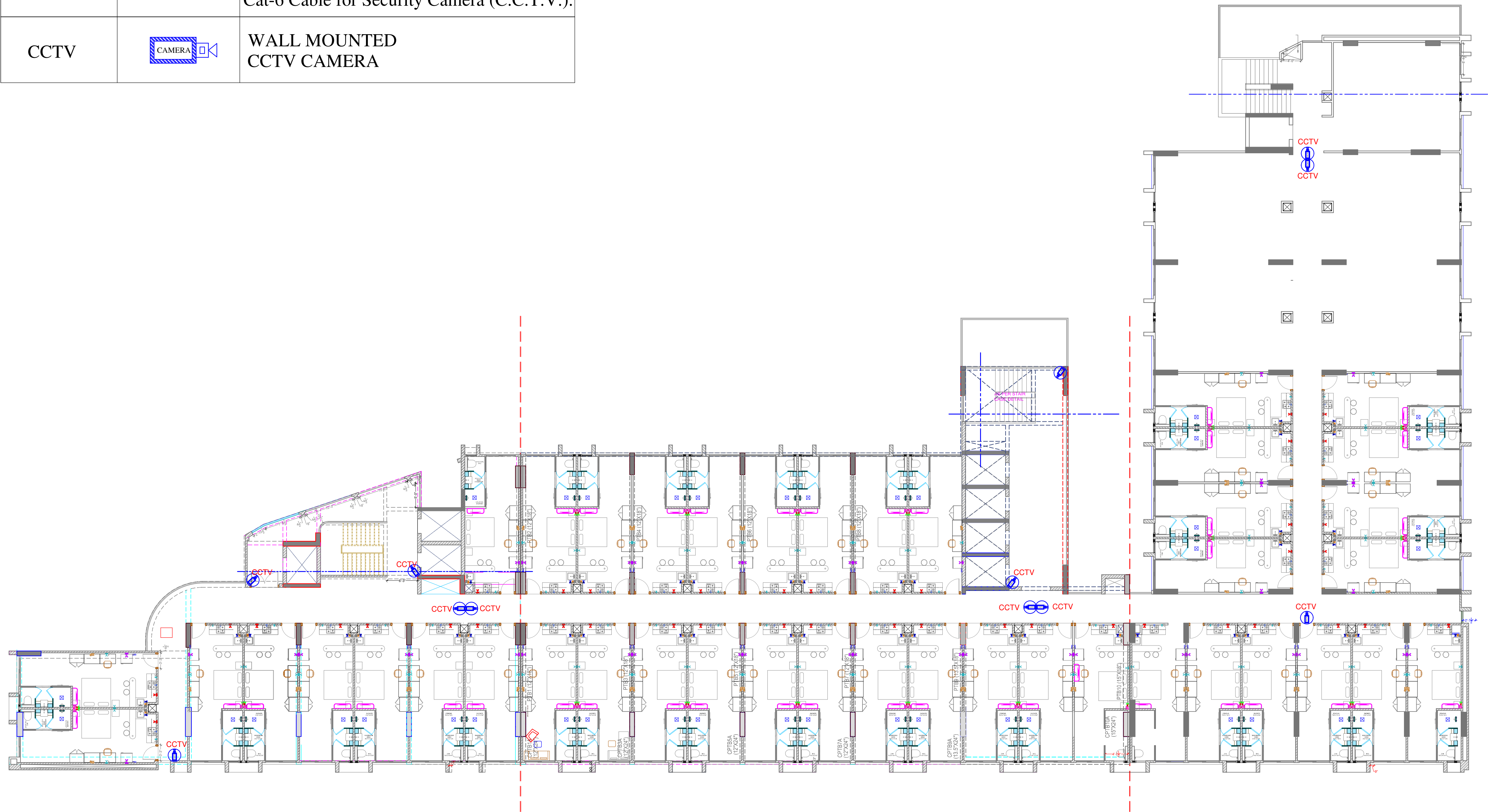
11th FLOOR WORKING PLAN
