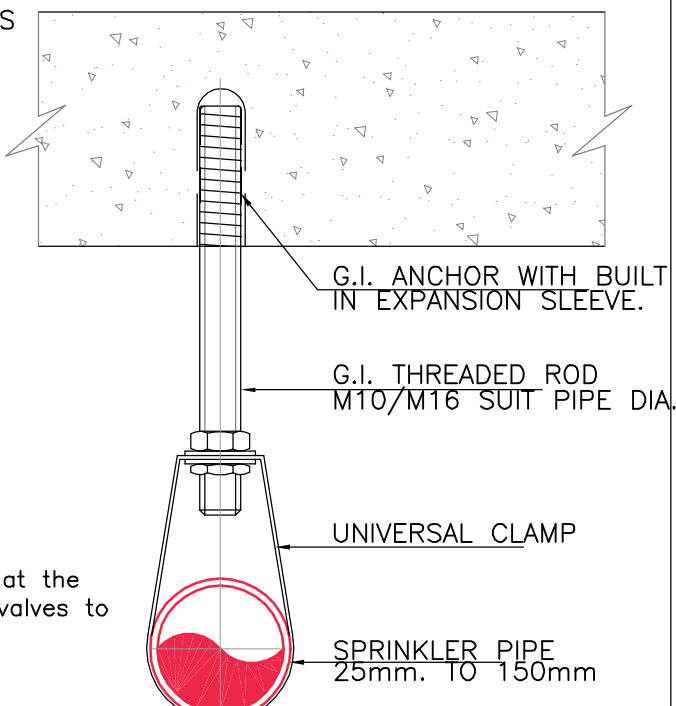
TYPICAL HANGING SUPPORT DETAILS FOR SPRINKLER / HYDRANT PIPES
