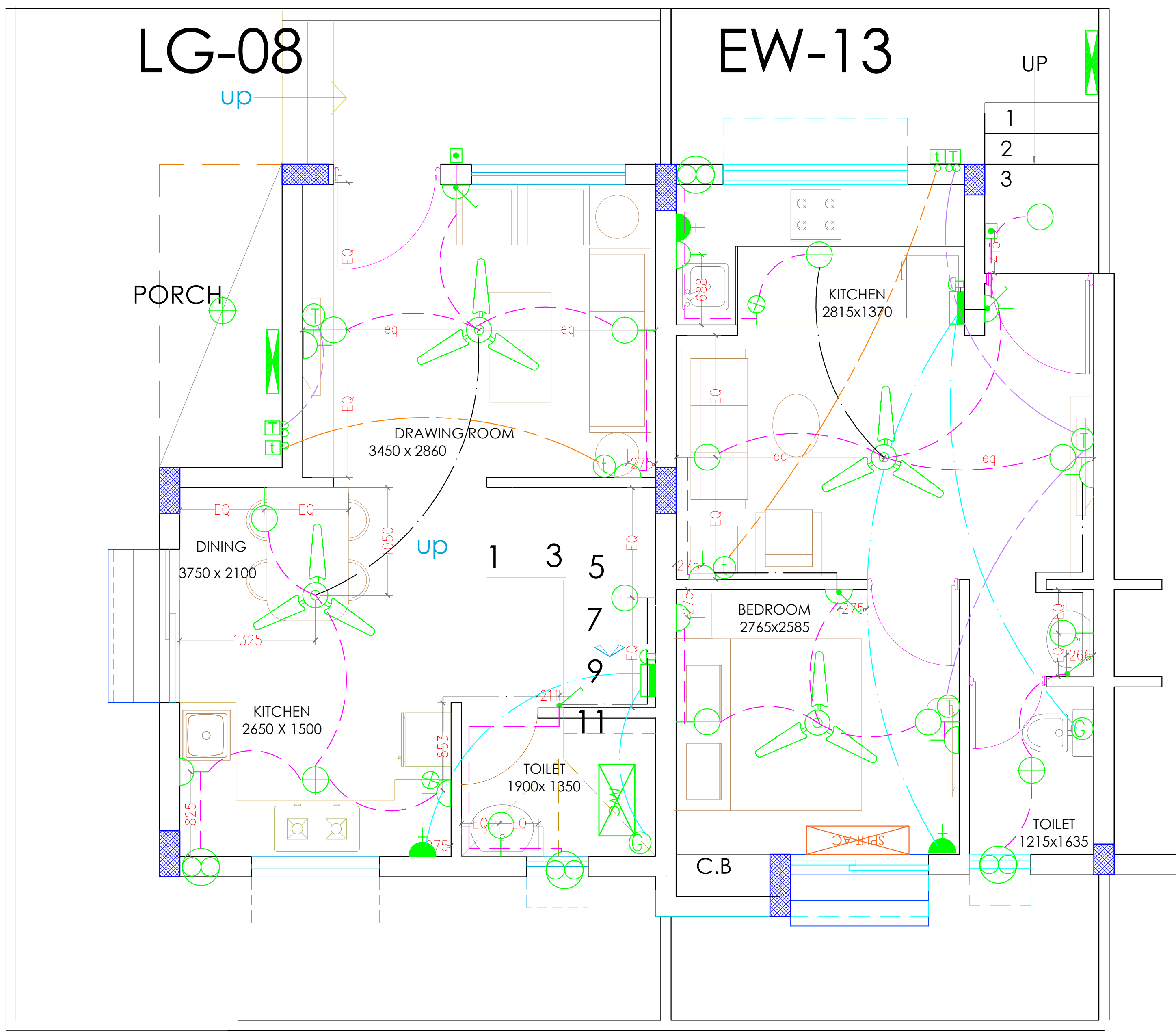
LG-08 EW-13 GROUND FLOOR PLAN
