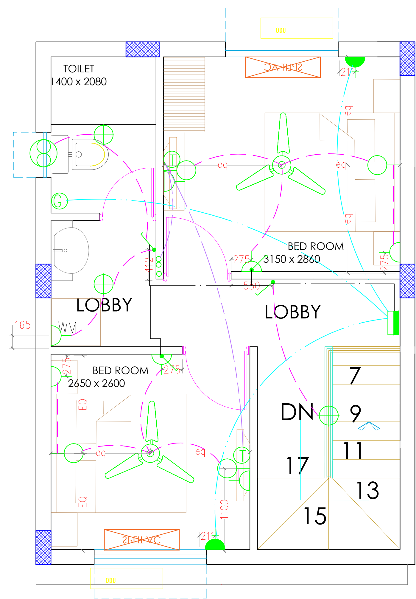
LG-08 FIRST FLOOR PLAN
