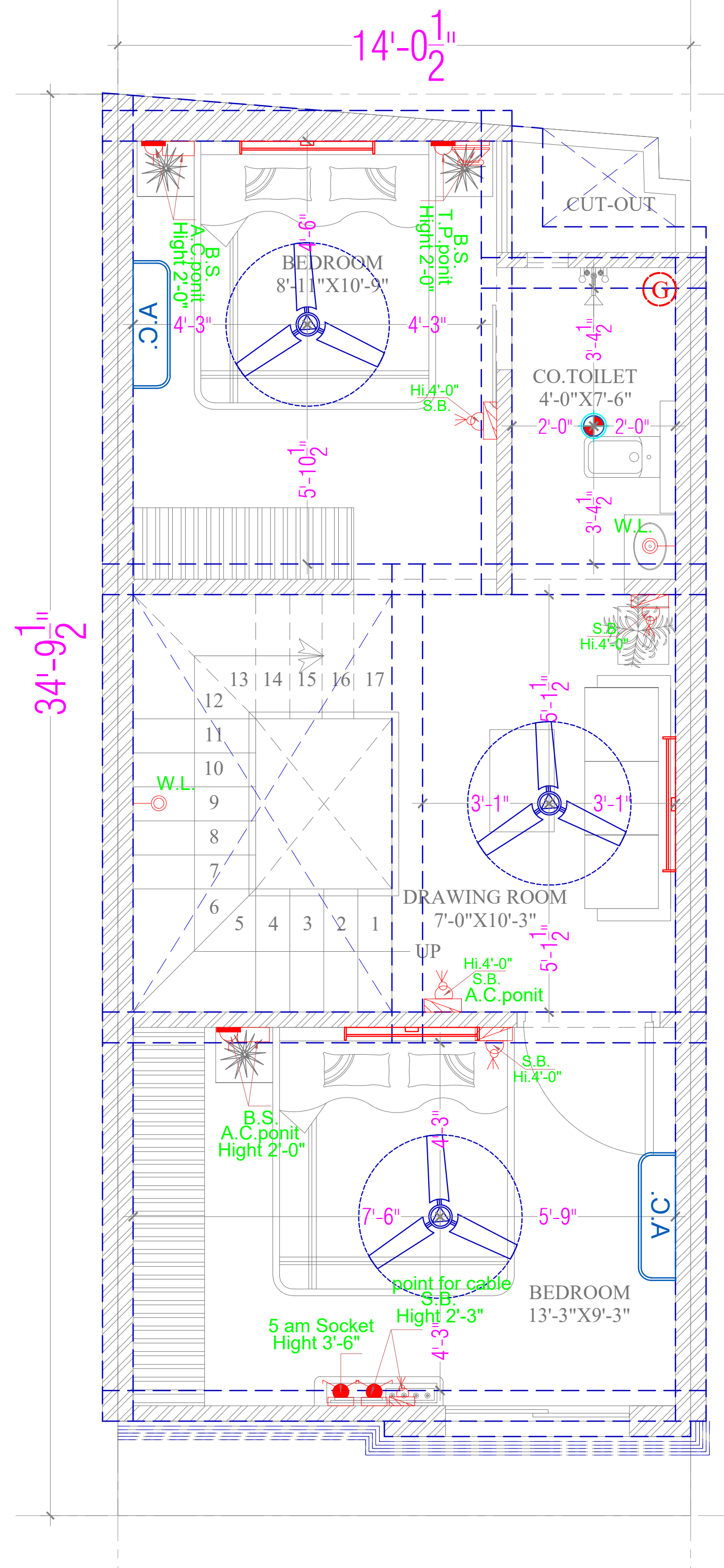
FIRST FLOOR ELECTRICAL PLAN
