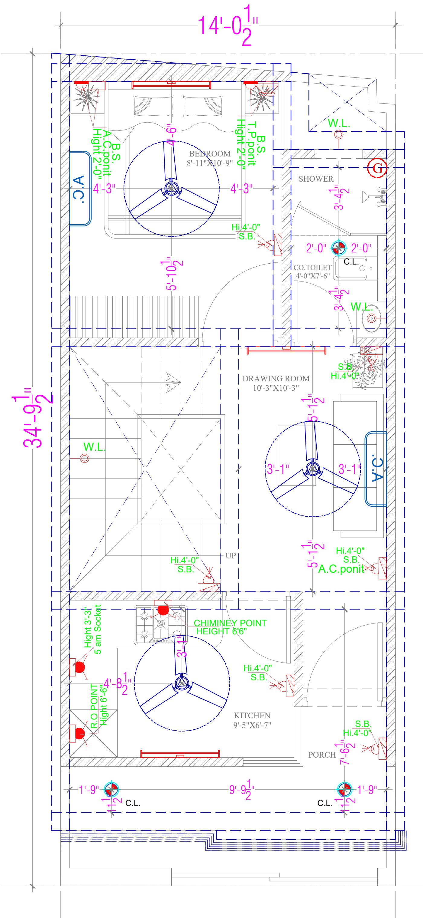
GROUND FLOOR ELECTRICAL PLAN
