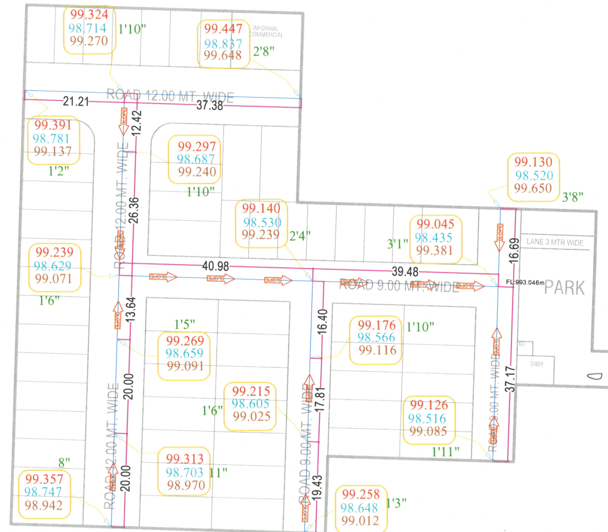
KEY PLAN
