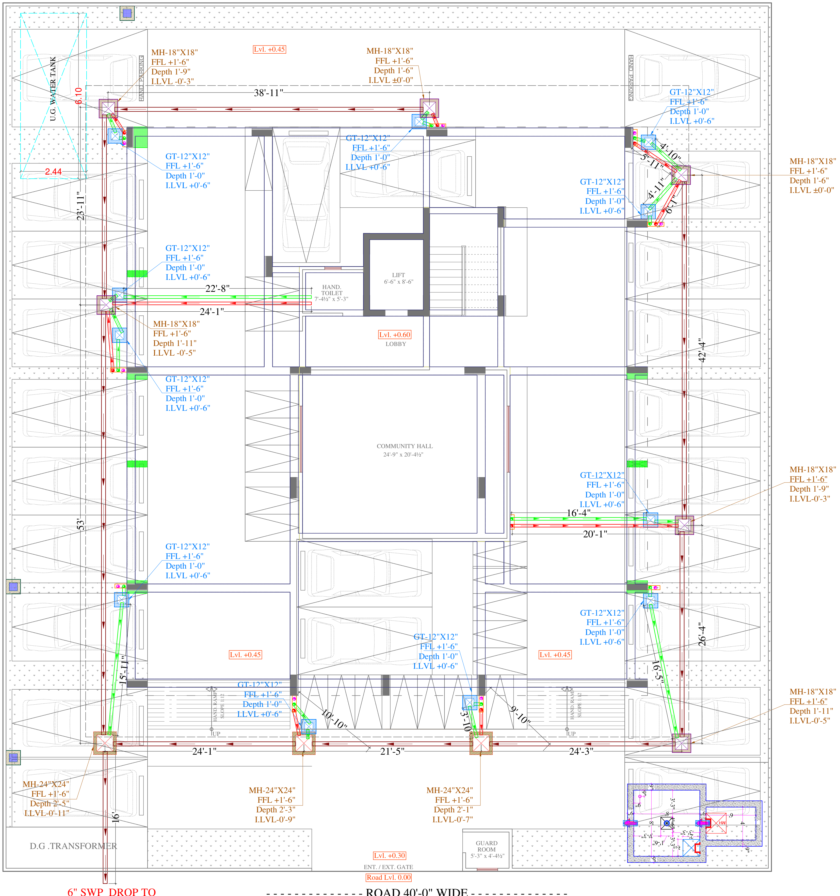
STILT FLOOR PLAN
