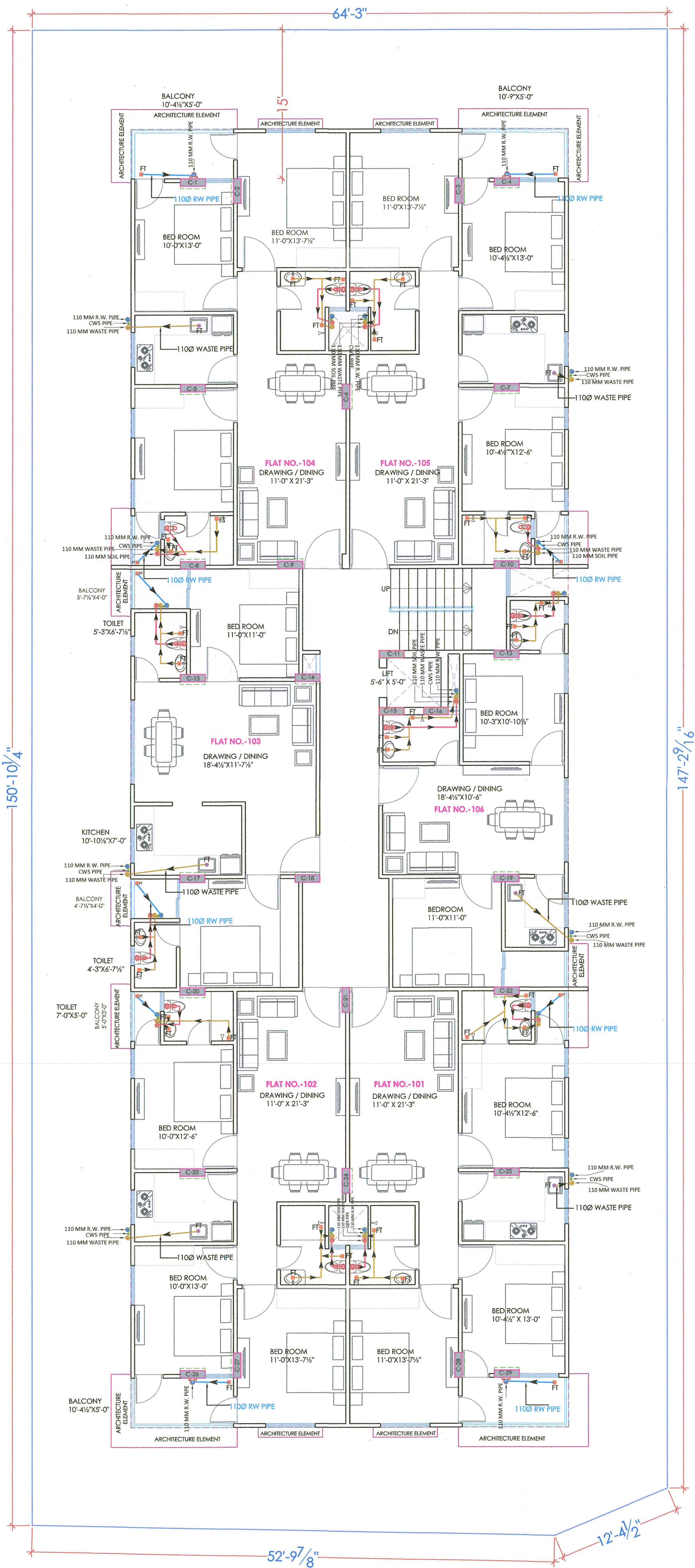
TYPICAL FLOOR (WATER SUPPLY, RAINWATER, SANITATION & COMMON PLUMBING ) DRAWING
