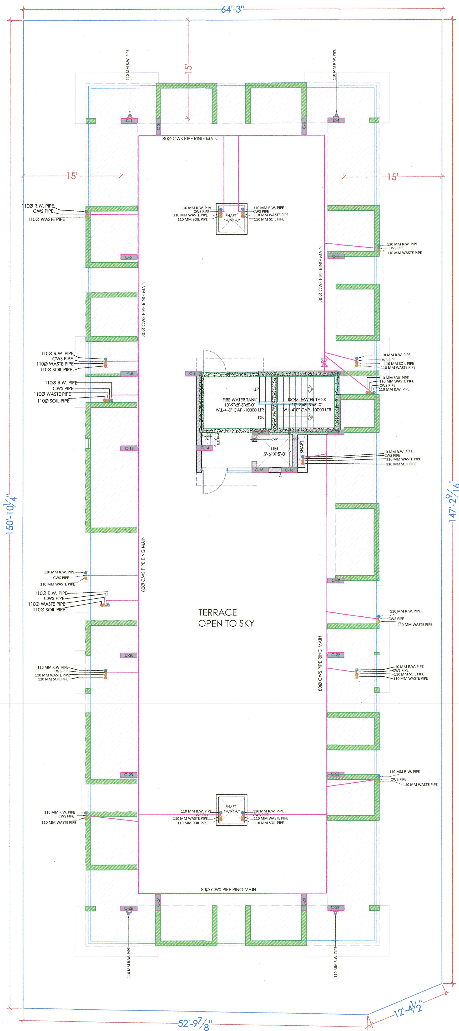
TERRACE FLOOR (WATER SUPPLY, RAINWATER, SANITATION & COMMON PLUMBING ) DRAWING
