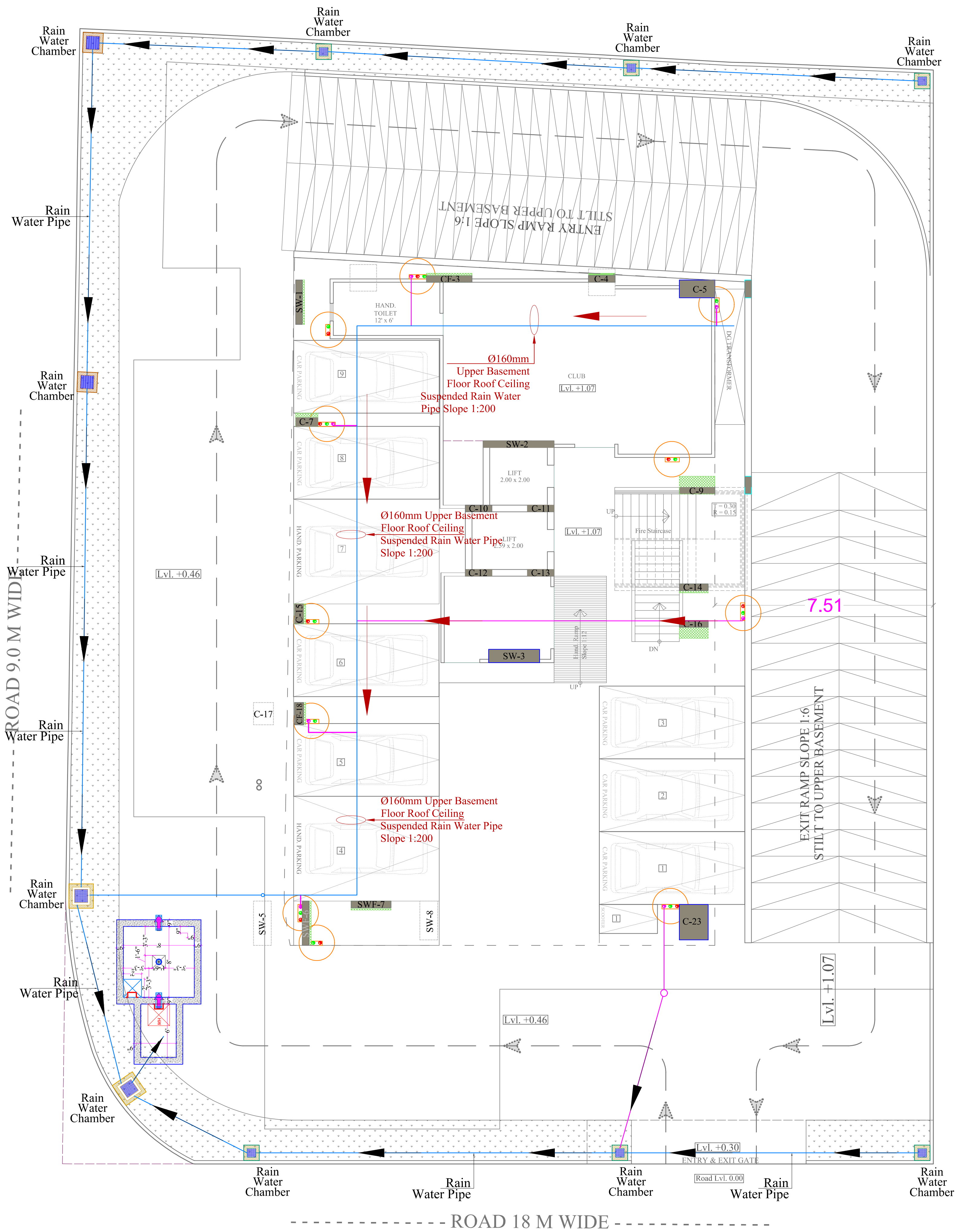
STILT PLAN WITH CIRCULATION
