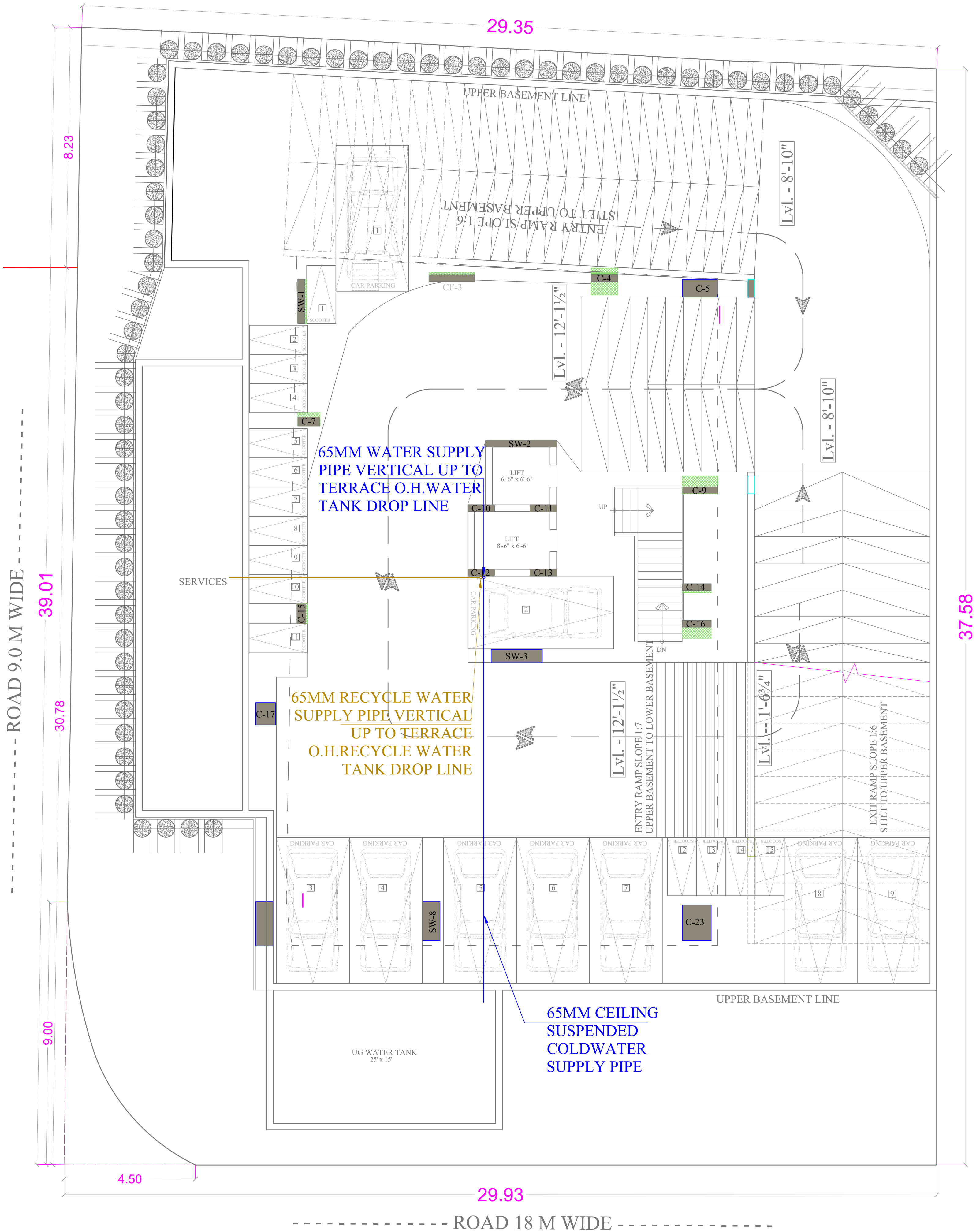
UPPER BASMENT PLAN WITH CIRCULATION
