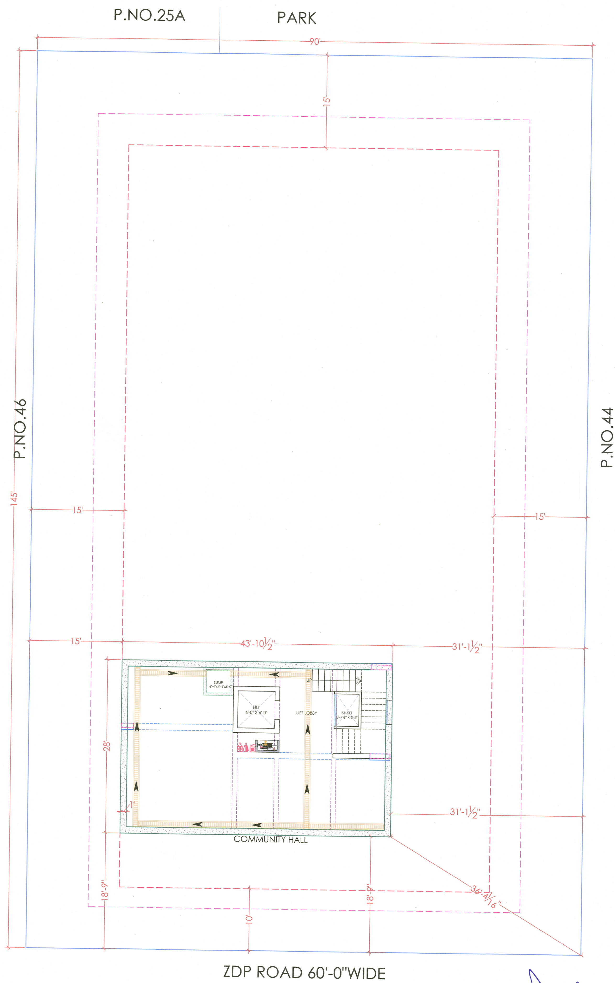
BASEMENT FLOOR FIRE FIGHTING LAYOUT
