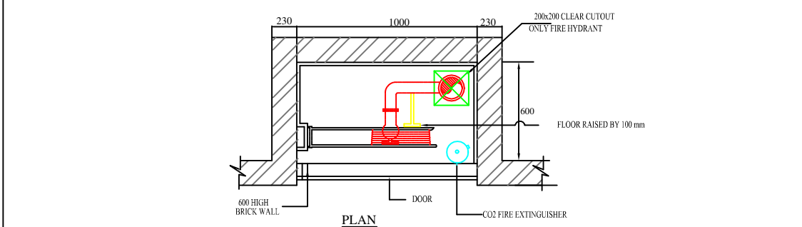
DRAWING: TYPICAL DETAIL FOR FIRE HOSE CABINET-1 SCALE=NTS [FHC-1]
