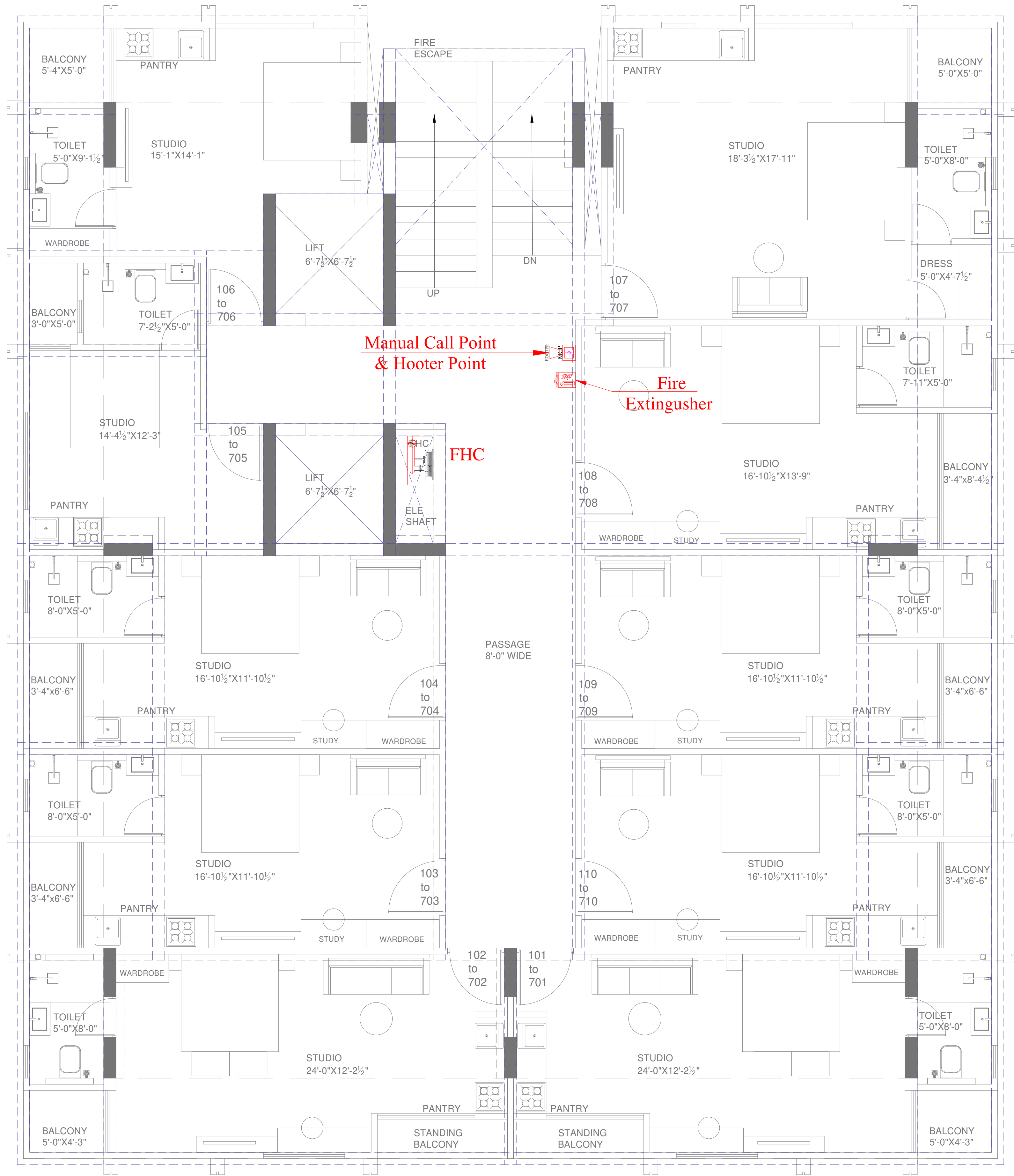
TYPICAL FIRST TO EIGHTH FLOOR PLAN
