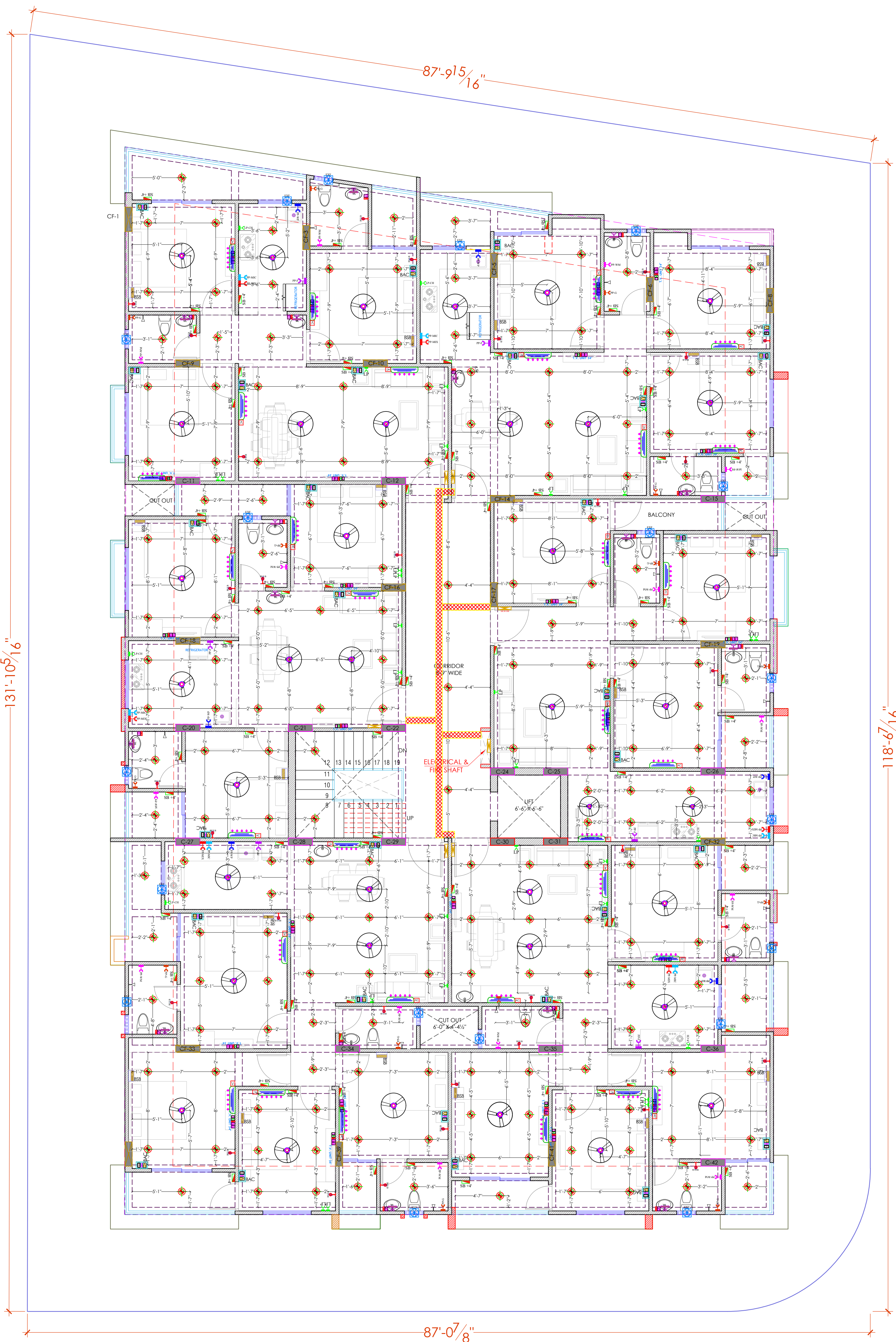
TYPICAL FLOOR G+4TH (ELECTRICAL POINT, CEILING POINT,TV)
