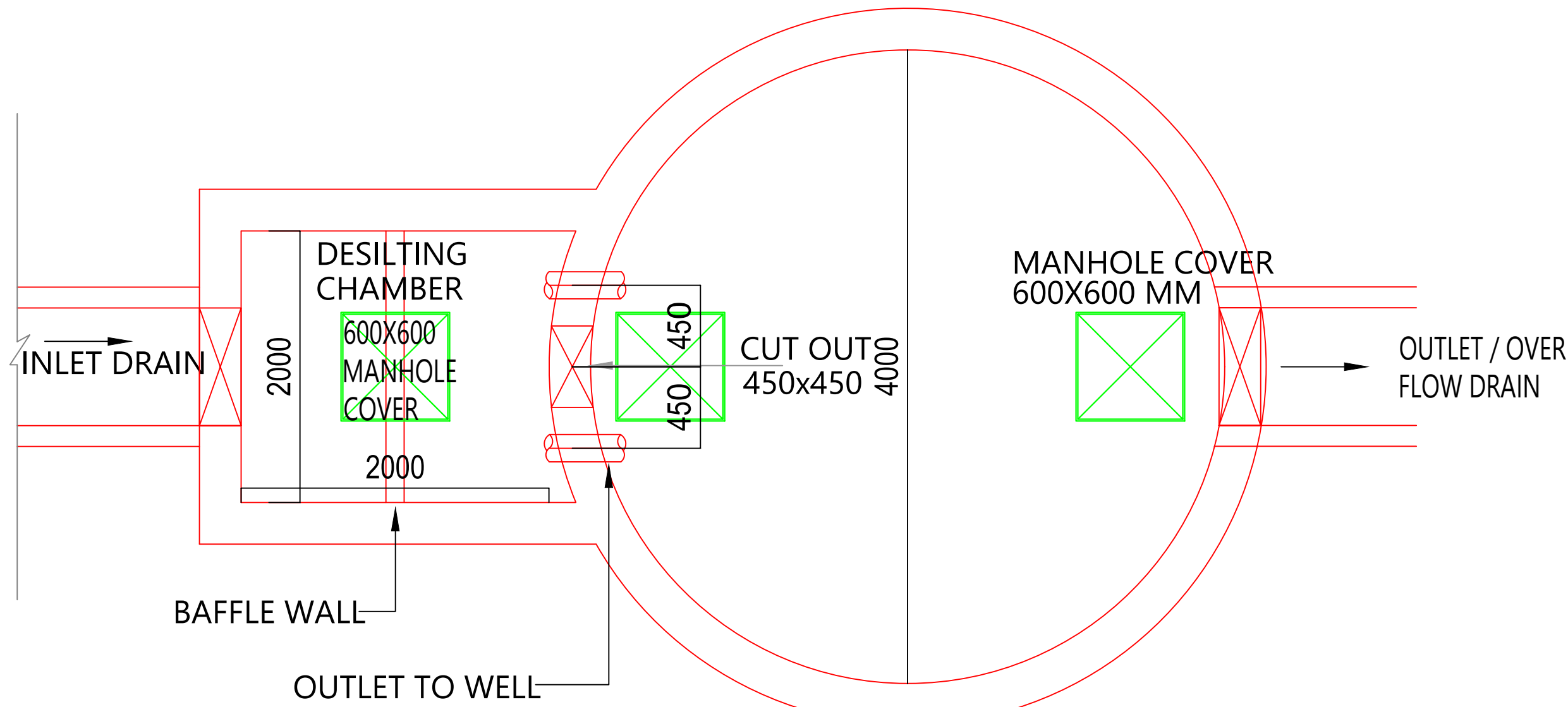
PLAN
