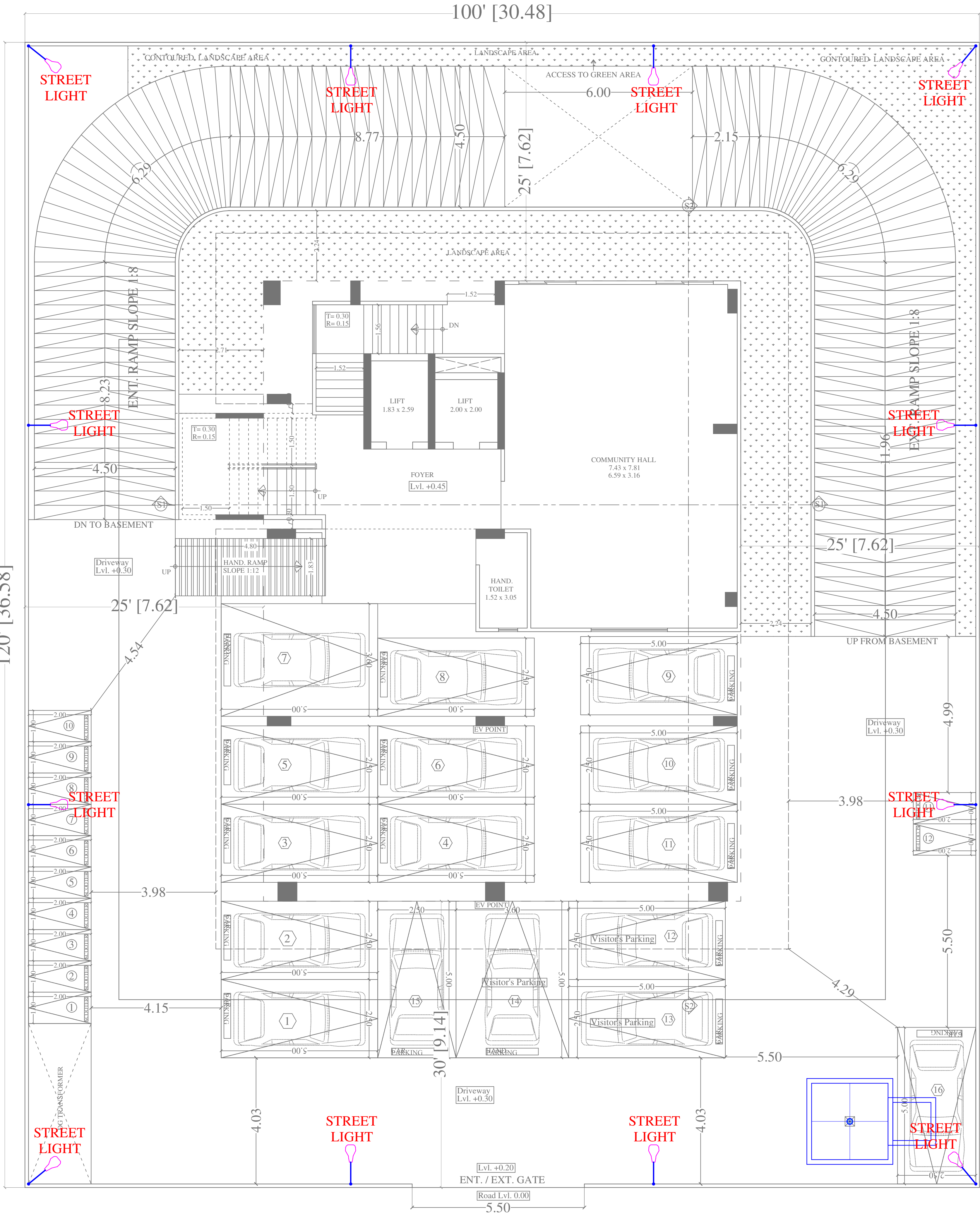
STILT PLAN
