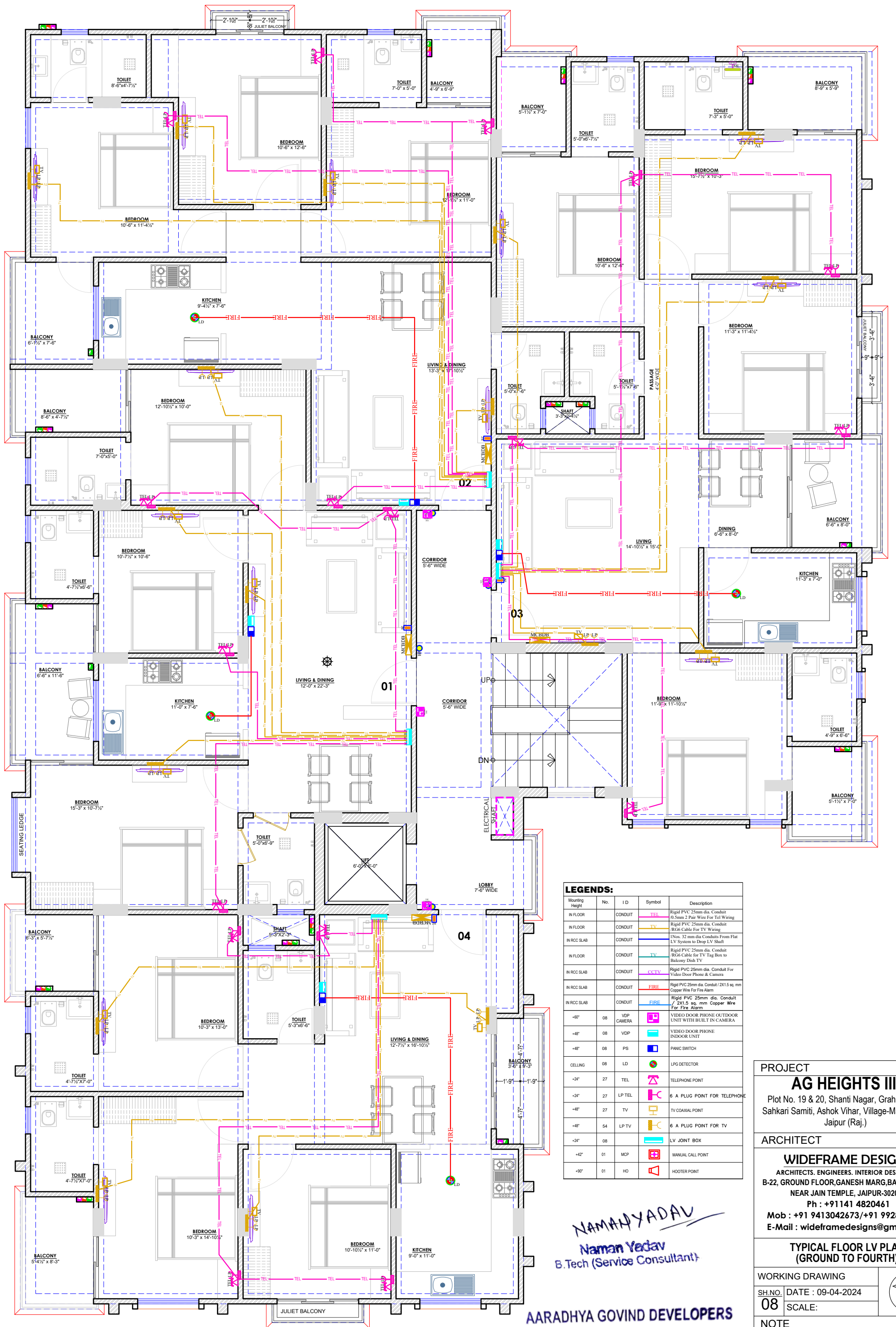
TYPICAL FLOOR LV PLAN (GROUND TO FOURTH)
