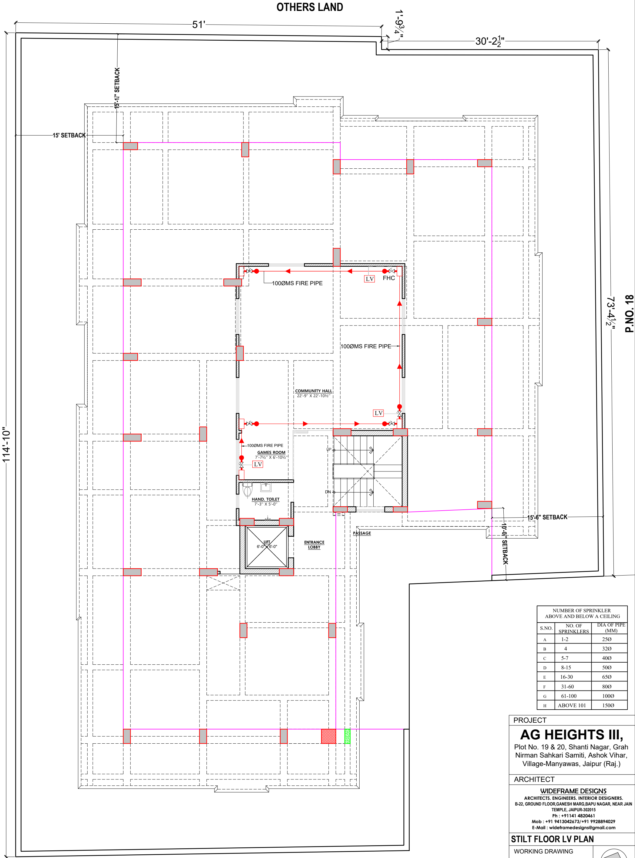
STILT FLOOR PLAN LV PLAN
