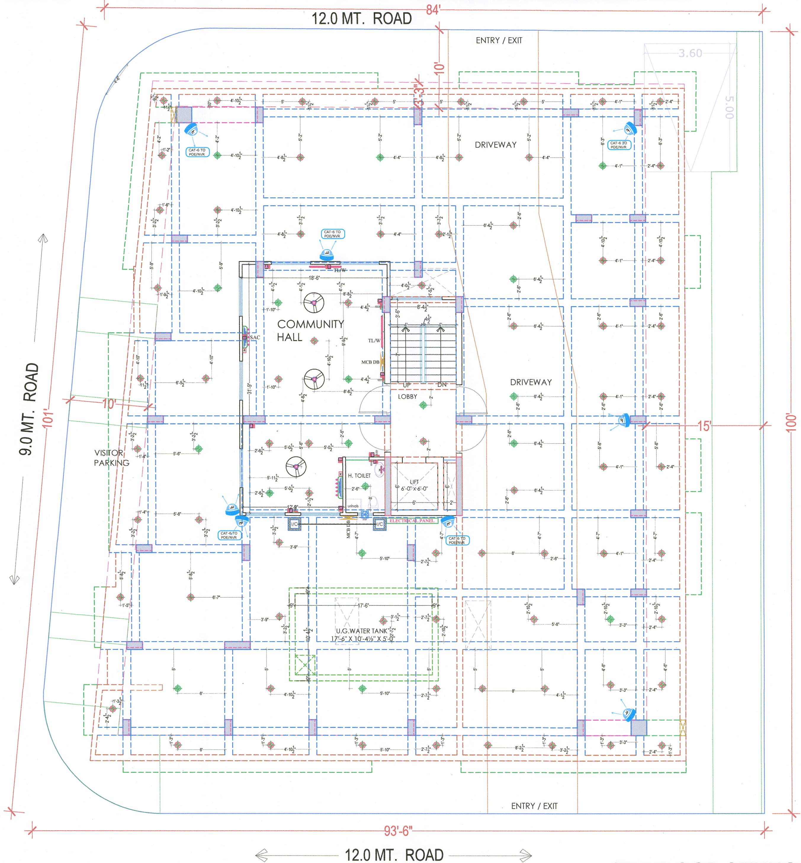
STILT FLOOR CEILING ELECTRICAL LAYOUT, ELECTRICAL POINT DRAWING
