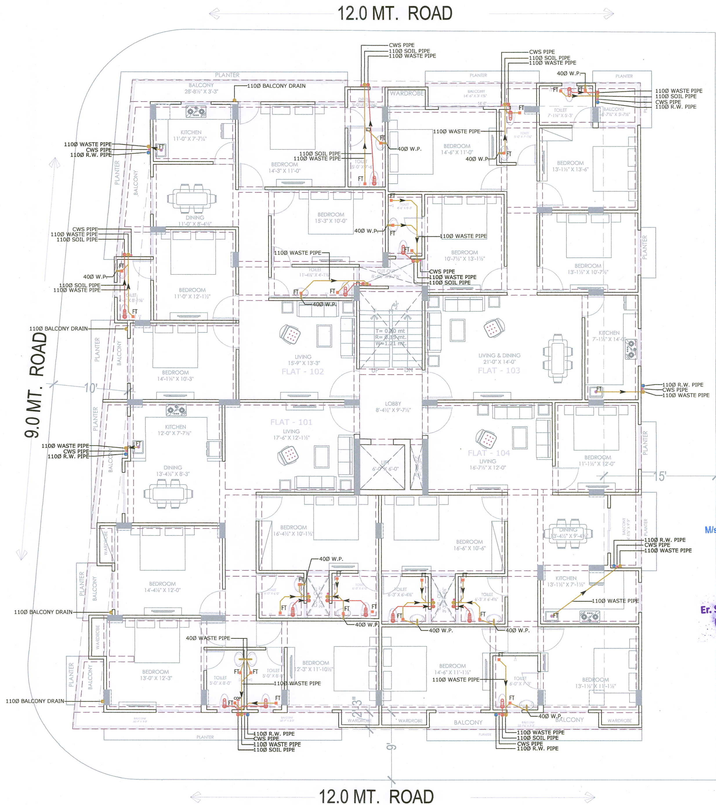
TYPICAL FLOOR (WATER SUPPLY, RAINWATER, SANITATION & COMMON PLUMBING ) DRAWING
