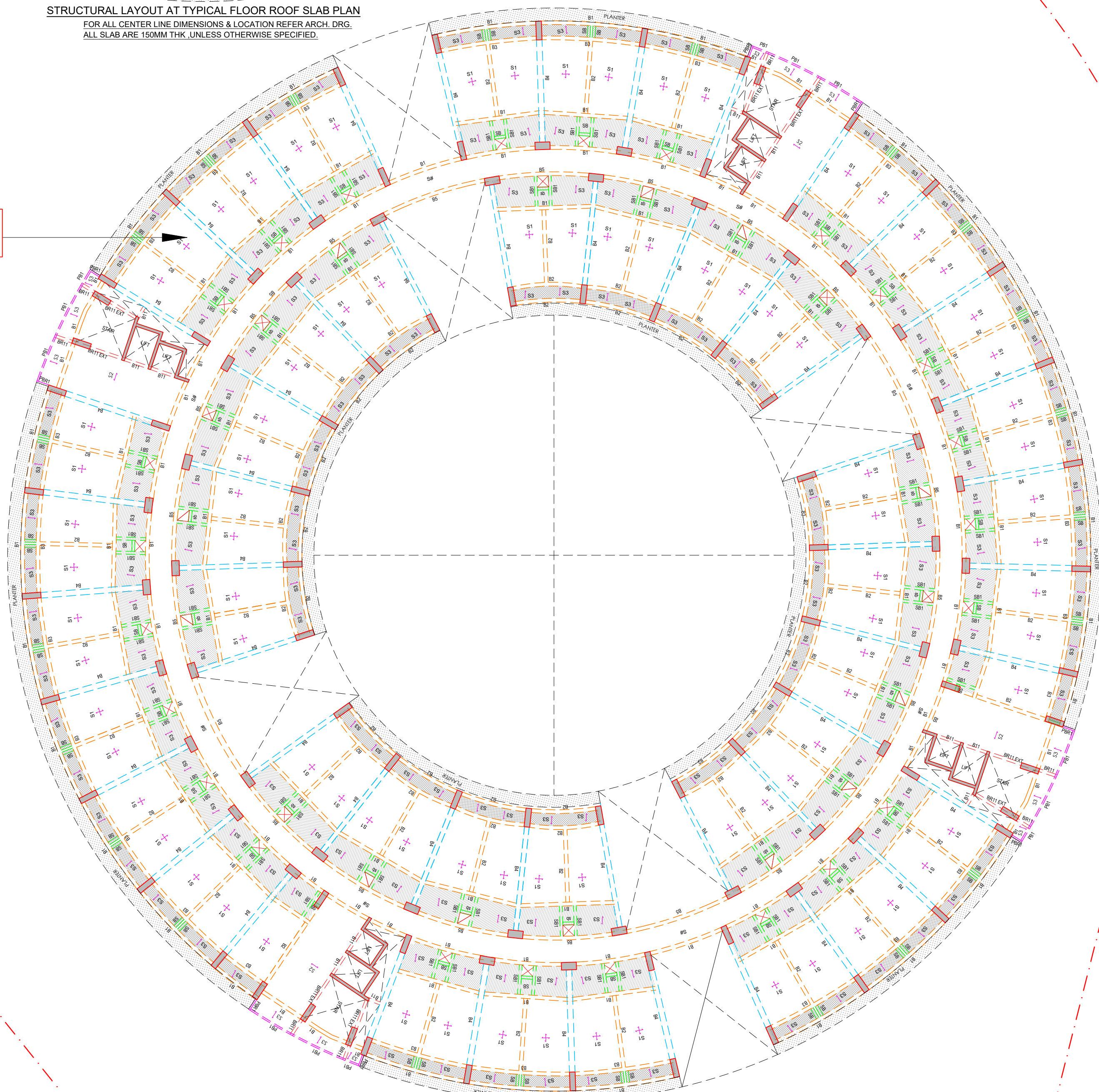
STRUCTURAL LAYOUT AT TYPICAL FLOOR ROOF SLAB PLAN FOR ALL CENTER LINE DIMENSIONS & LOCATION REFER ARCH. DRG. ALL SLAB ARE 150MM THK ,UNLESS OTHERWISE SPECIFIED.
