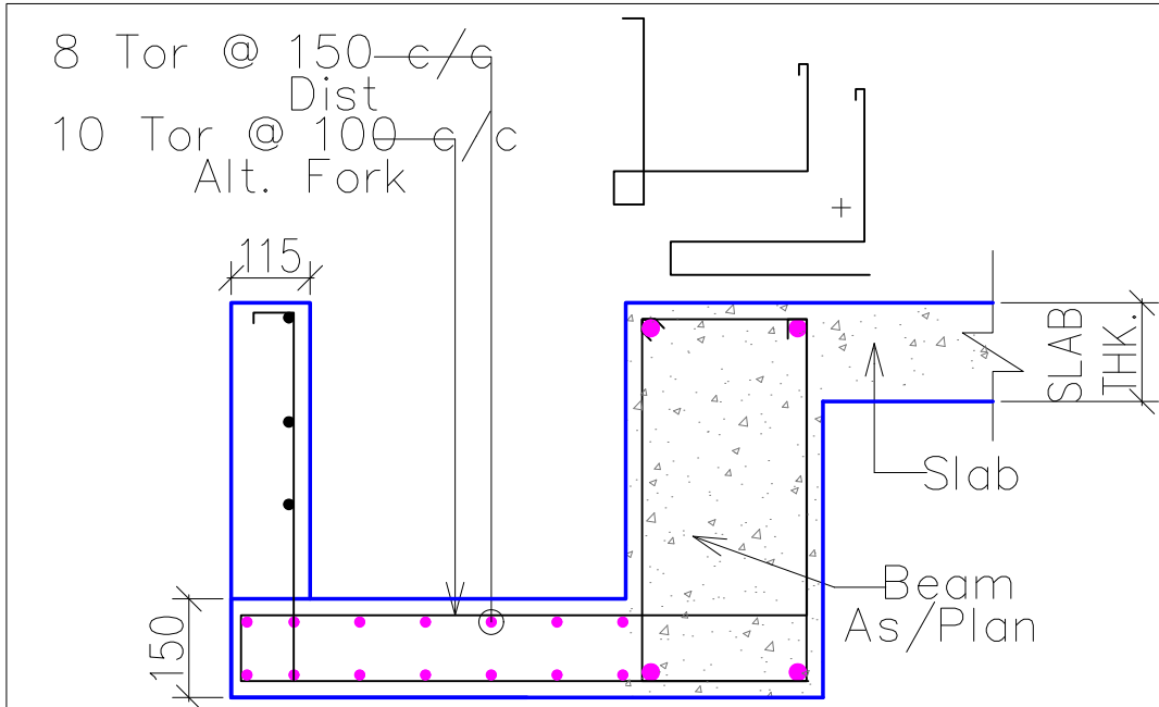
TYPICAL PLANTER SECTION
