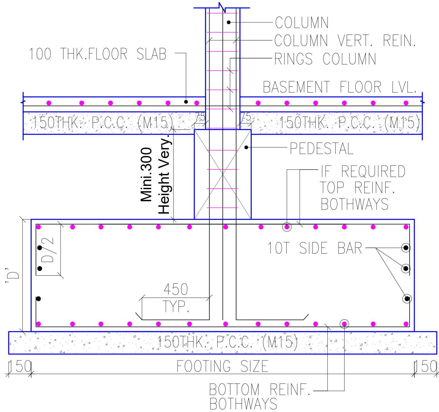
TYPICAL FOOTING SECTION BOX&RAFT FOOTING
