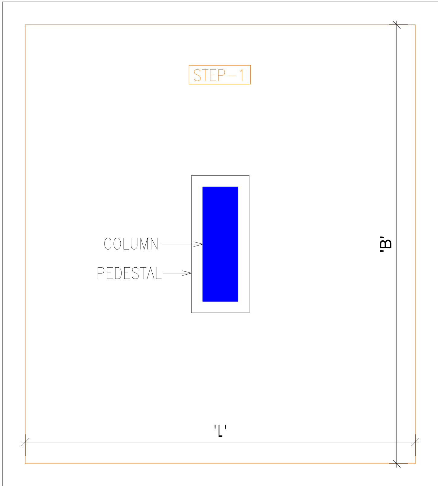
TYPICAL BOX FOOTING PLAN
