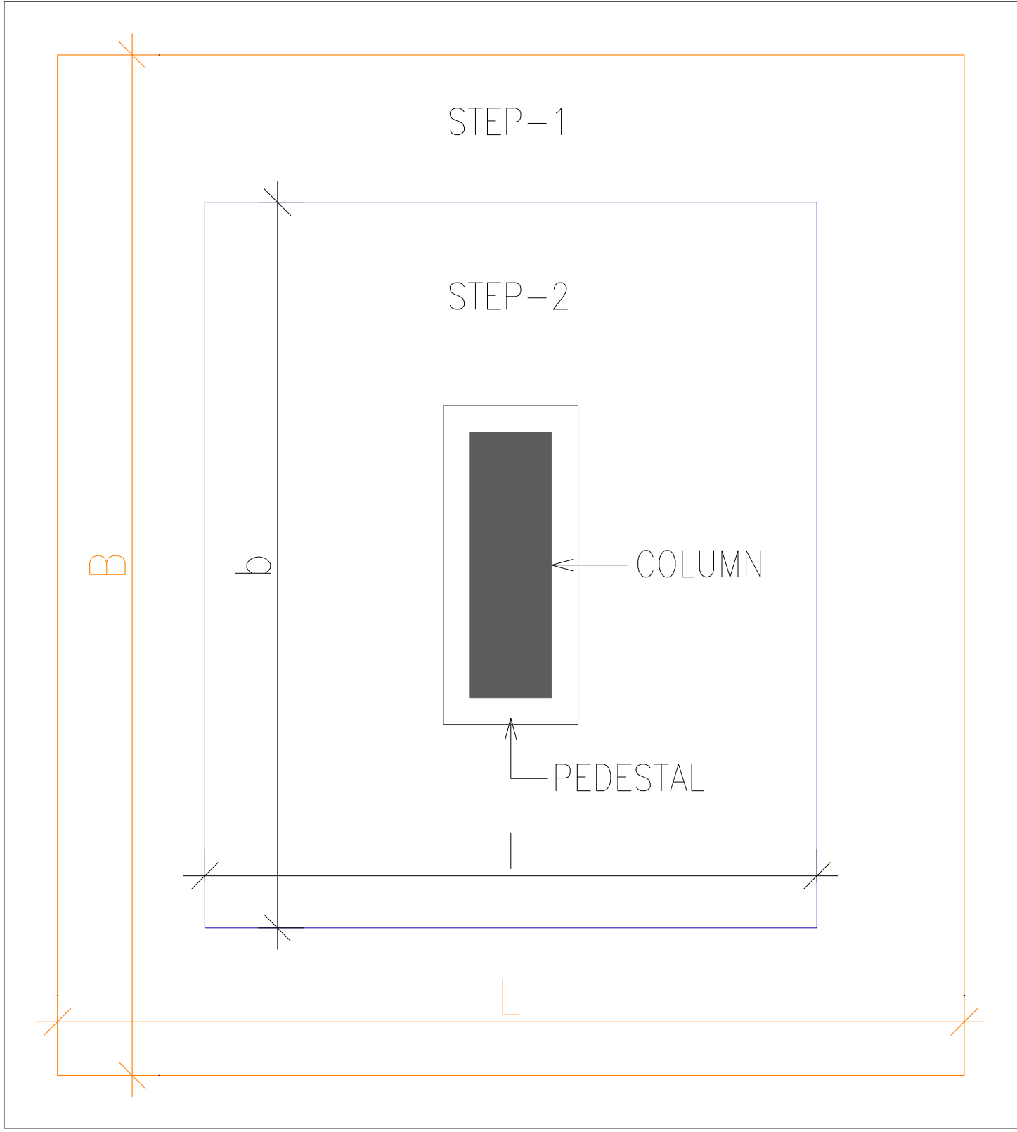
TYPICAL STEP FOOTING PLAN
