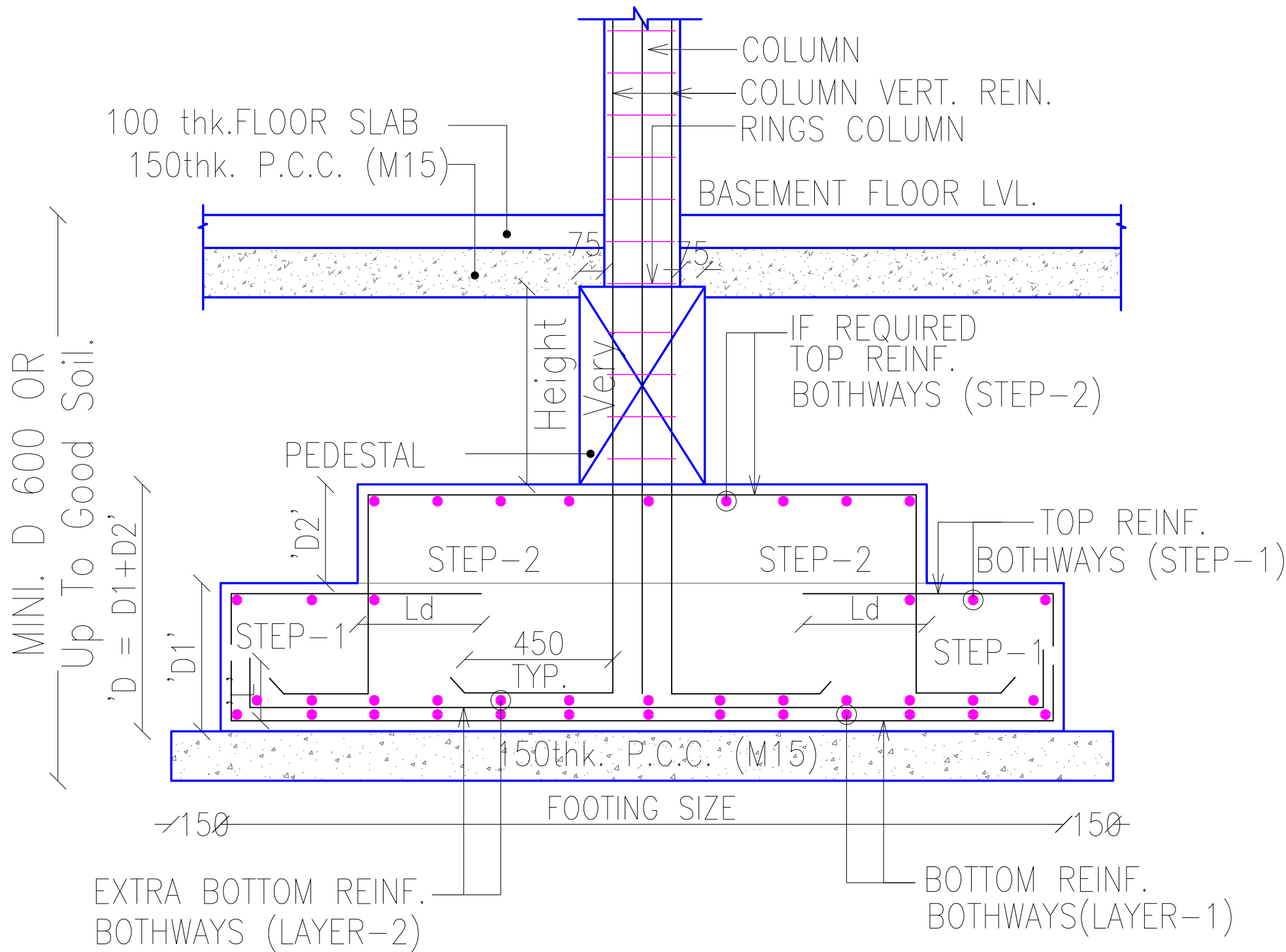
TYPICAL STEP FOOTING SECTION
