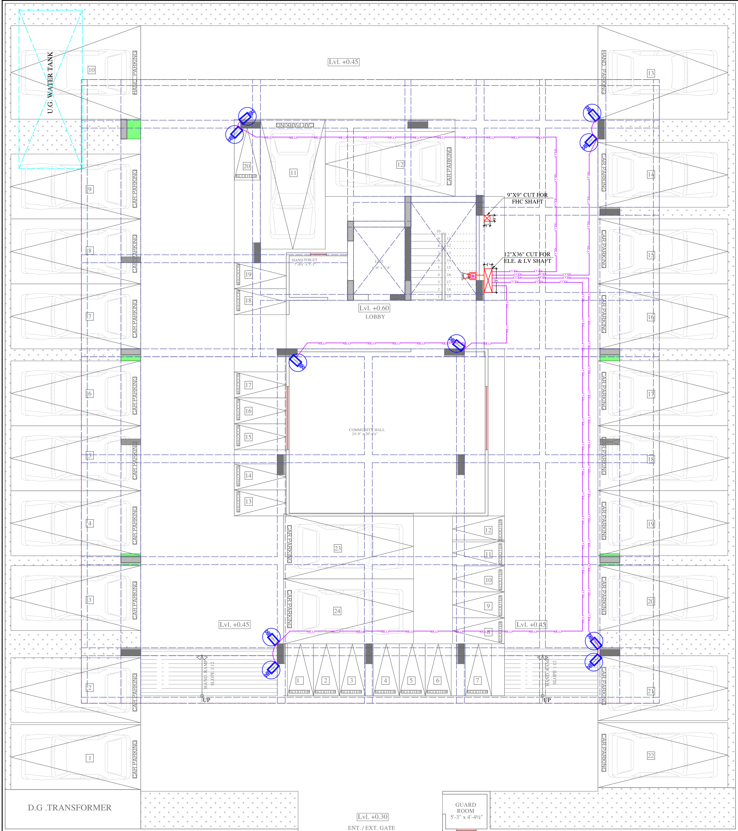
STILT PLAN
