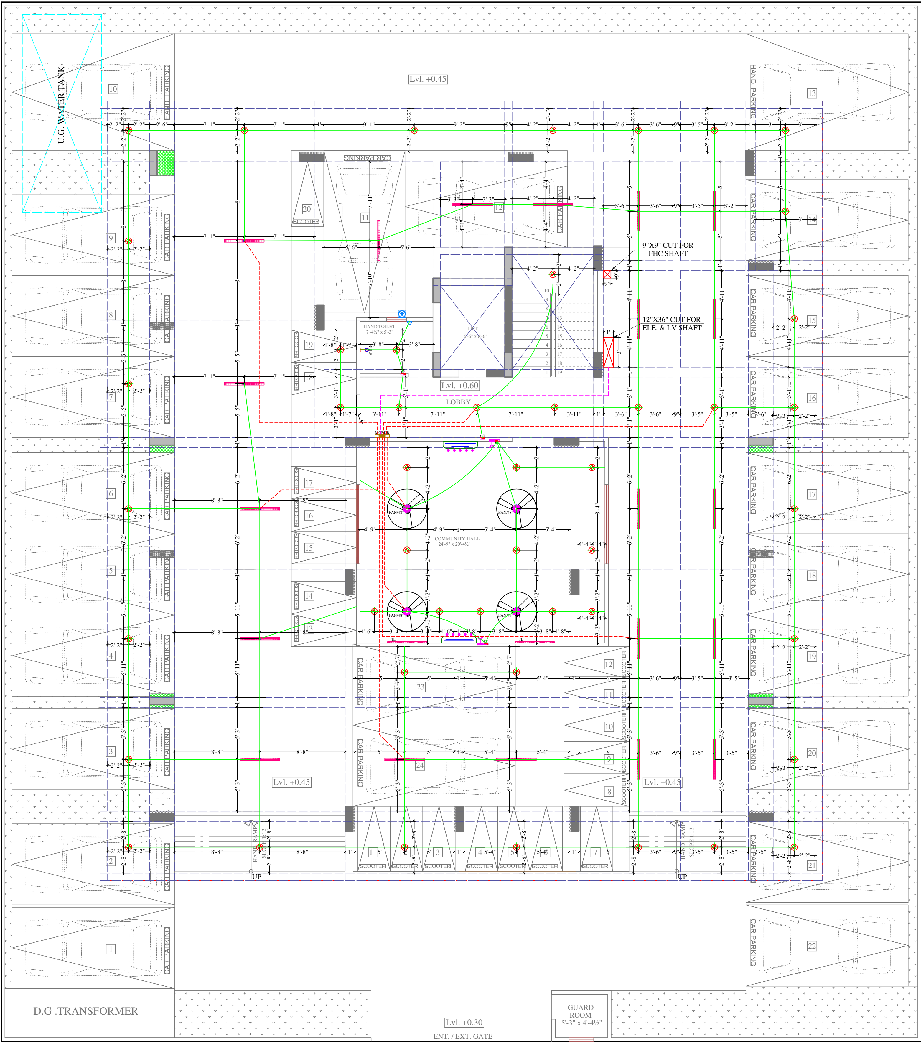
STILT PLAN
