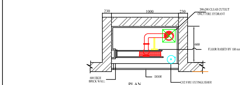
DRAWING: TYPICAL DETAIL FOR FIRE HOSE CABINET-1 SCALE=NTS FHC-1
