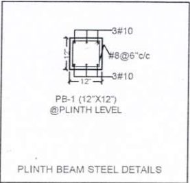
PLINTH BEAM STEEL DETAILS
