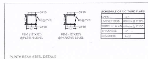
PLINTH BEAM STEEL DETAILS
