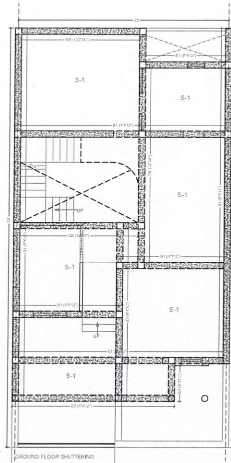
GROUND FLOOR SHUTTERING
