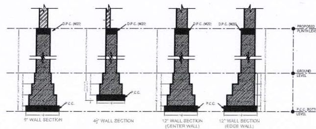
FOUNDATION SECTION DETAILS
