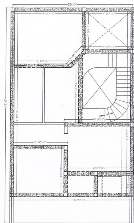
FIRST FLOOR SHUTTERING
