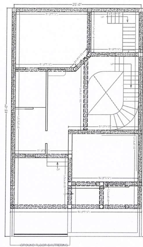
GROUND FLOOR SHUTTERING
