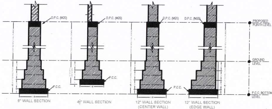
FOUNDATION SECTION DETAILS
