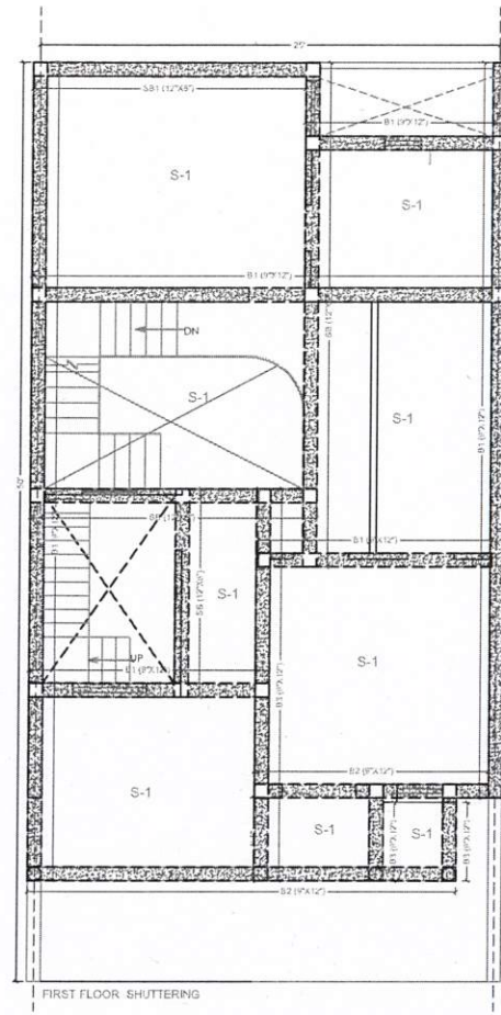
FIRST FLOOR SHUTTERING
