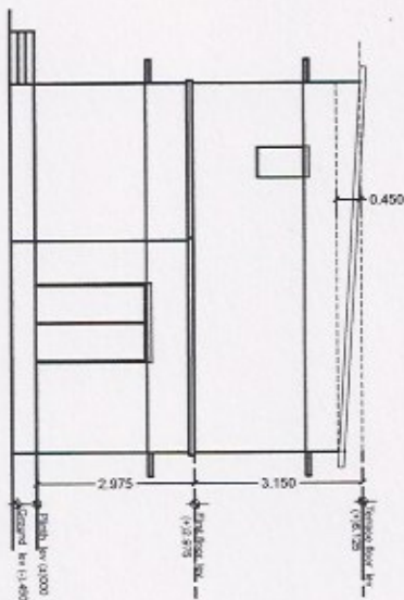
SIDE ELEVATION - 1
