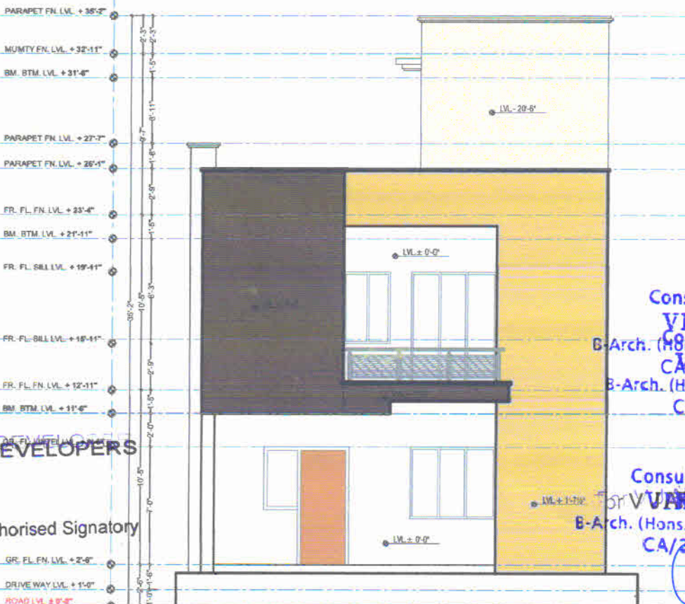
REAR ELEVATION
