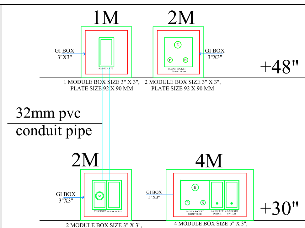
1M 2M 32mm pvc conduit pipe 2M 4M
