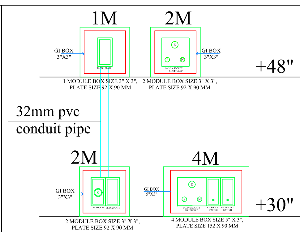
TYPICAL TV WALL ELEVATION PLAN
