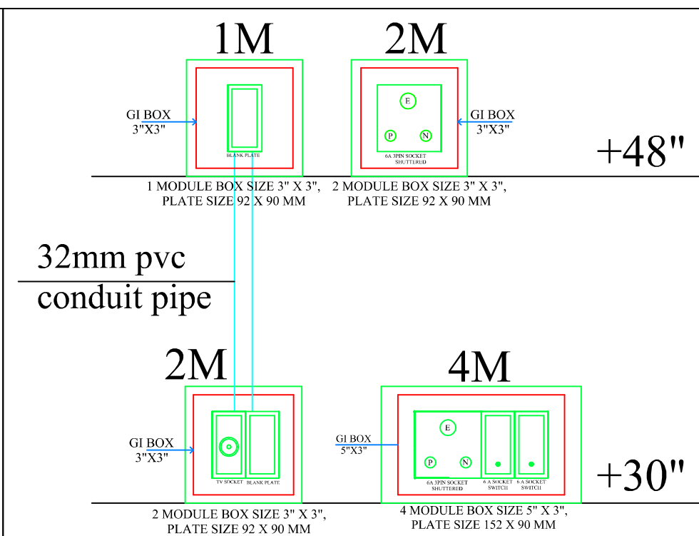
TYPICAL TV WALL ELEVATION PLAN
