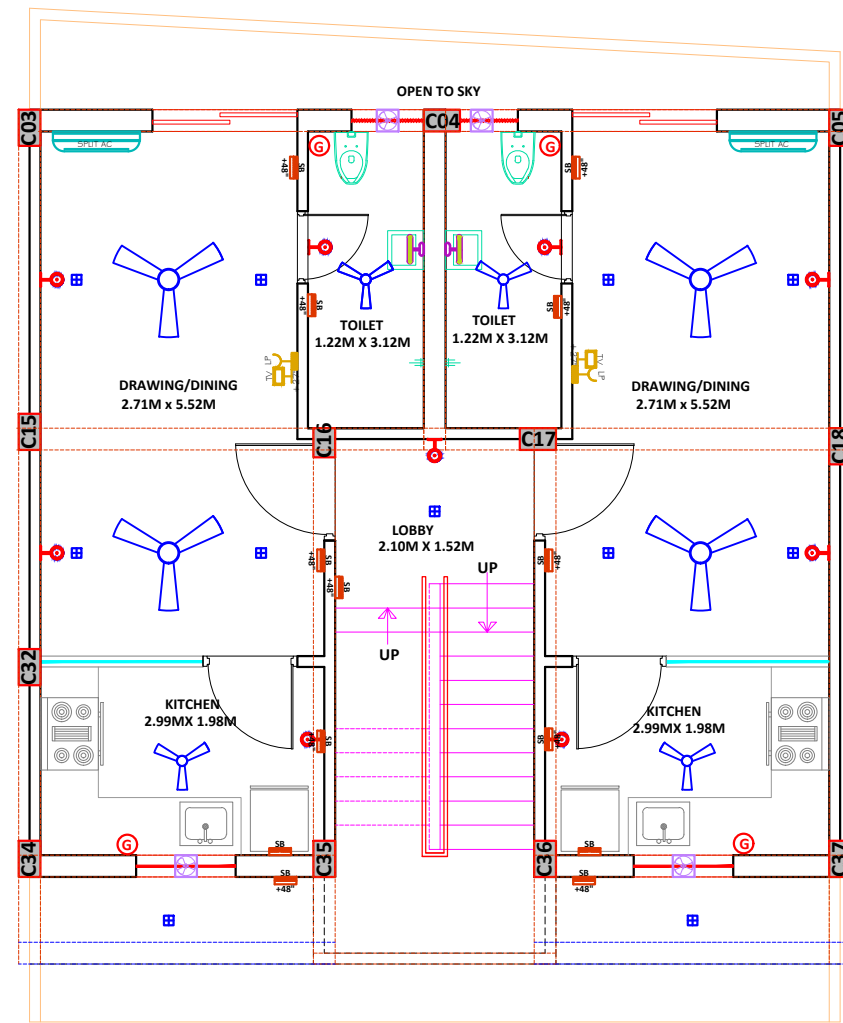
54 55 GROUND FLOOR PLAN
