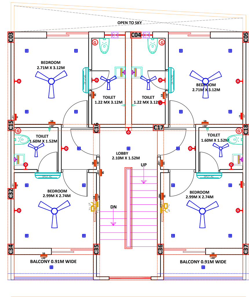
54 55 FIRST FLOOR PLAN
